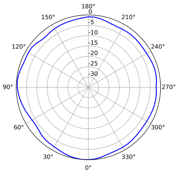
2.4G (Horizontal)
