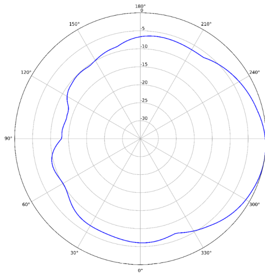
2.4GHz (Horizontal)
