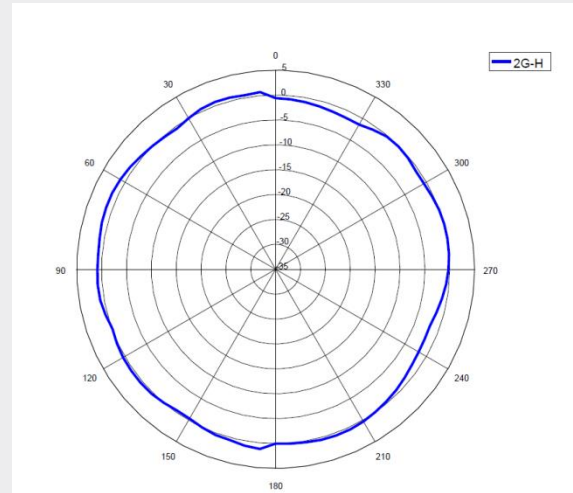
2.4G (PHI=90)
