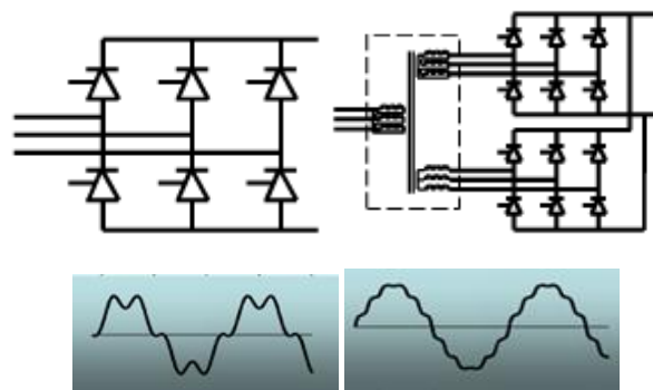
Figure 1 6-pulse and 12-pulse circuits and current waveforms
