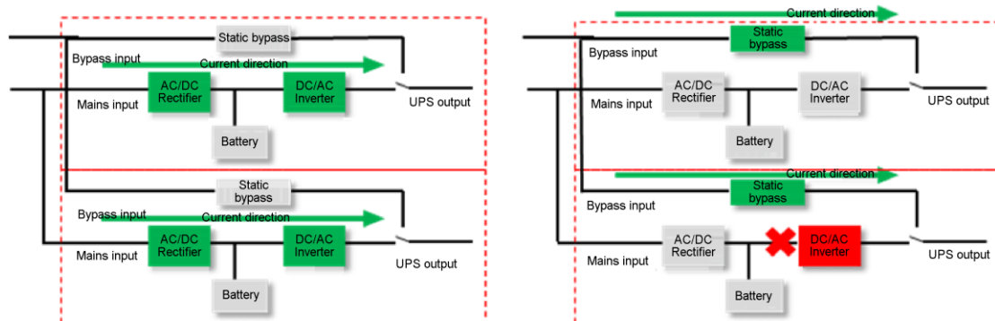
Figure 2 UPS parallel system in the bypass mode
