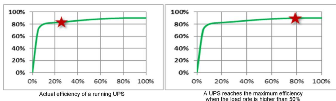
Figure 4 Actual efficiency and maximum efficiency of the UPS system
