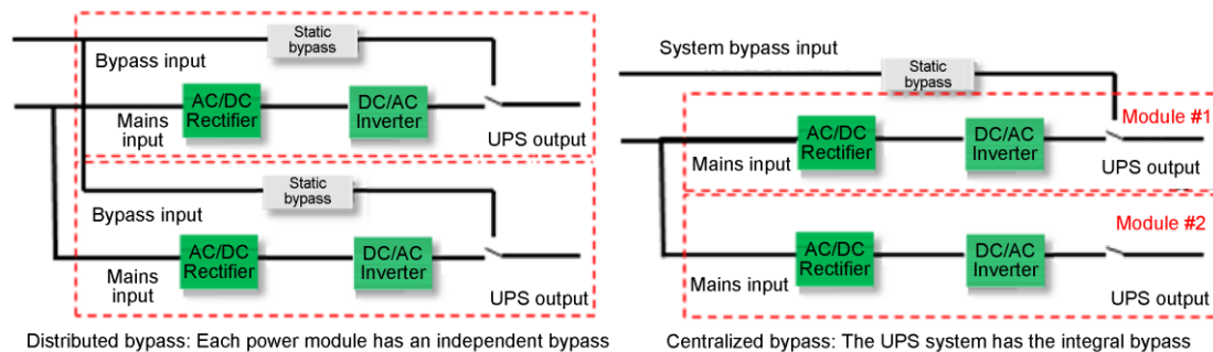
Figure 6 Distributed bypass and centralized bypass
