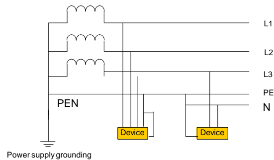
Figure 5 TN-C-S system grounding
