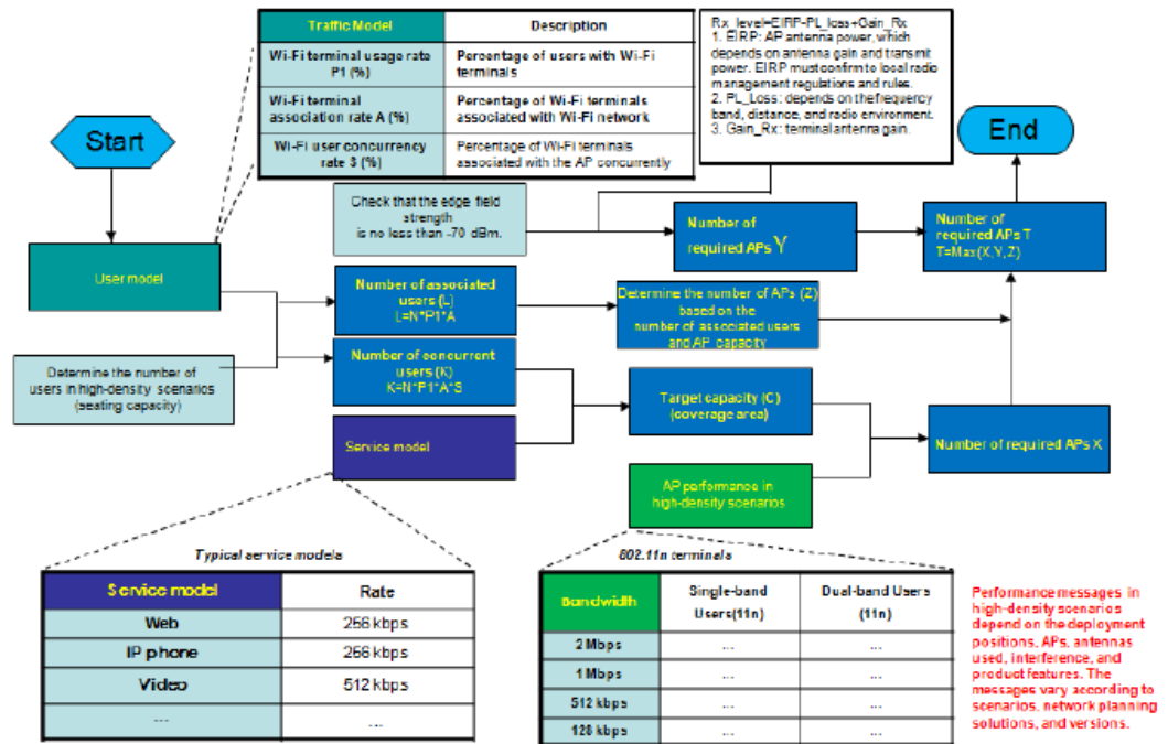
Figure 2-15 AP quantity calculation process
