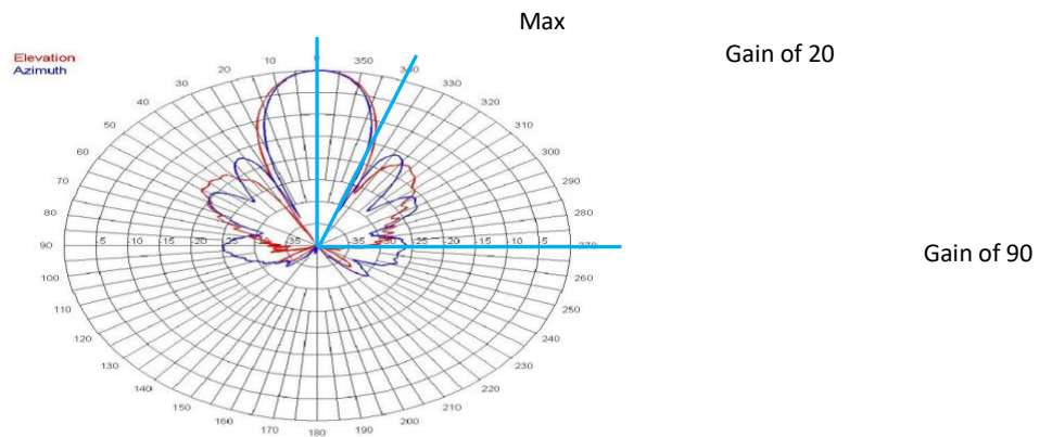
Figure 2-5 Huawei 18-degree antenna used in high-density scenarios
