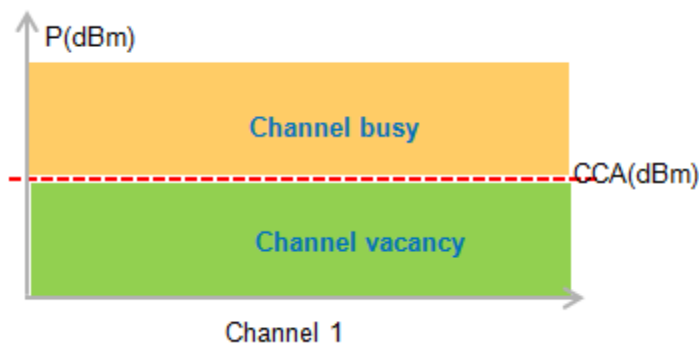
Figure 2-6 CCA principles
