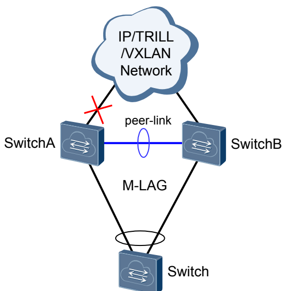
Figure 1-27 Uplink fails
