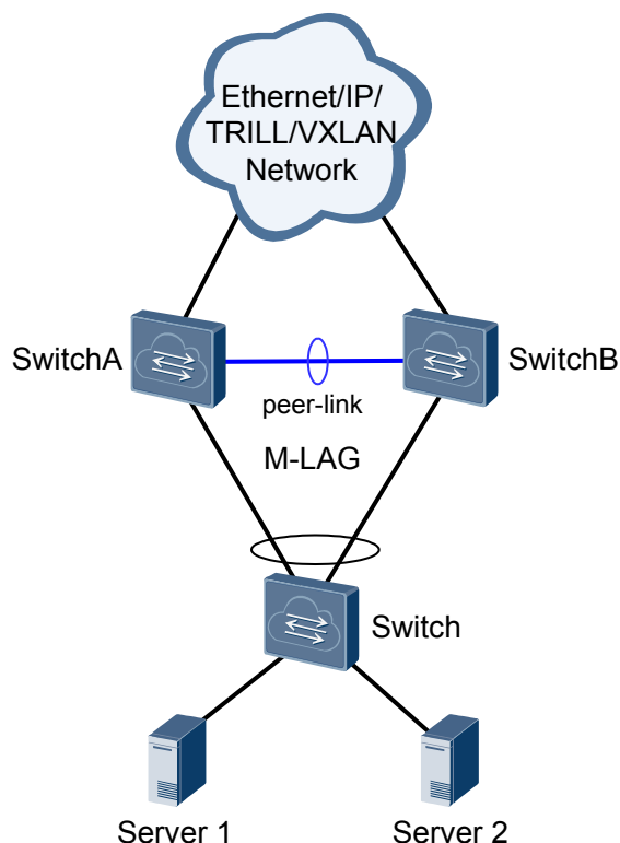
Figure 1-24 Connecting a switch in dual-homing mode
