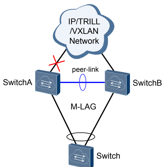
Figure 1-28 Uplink fails
