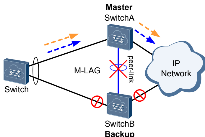
Figure 1-20 Peer-link fails
