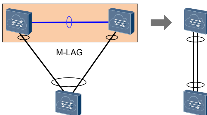
Figure 1-1 M-LAG network
