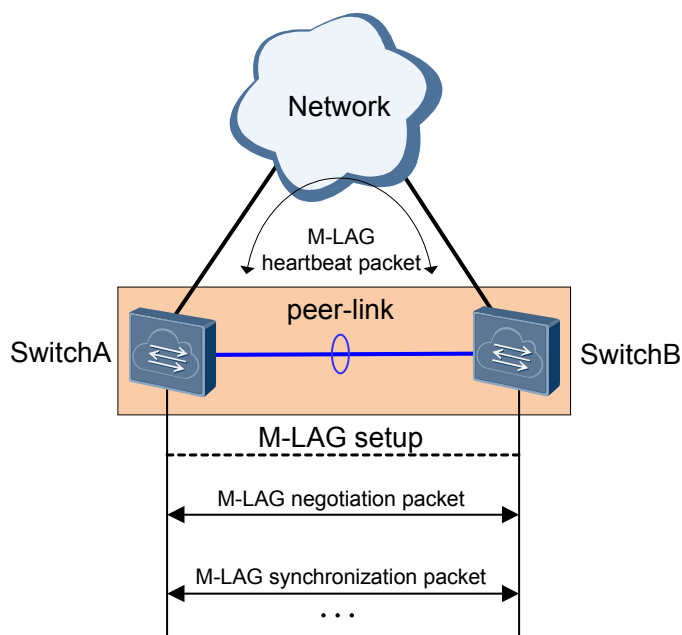
Figure 1-3 M-LAG setup
