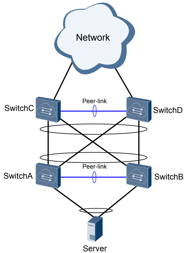
Figure 1-26 Networking of multi-level M-LAG
