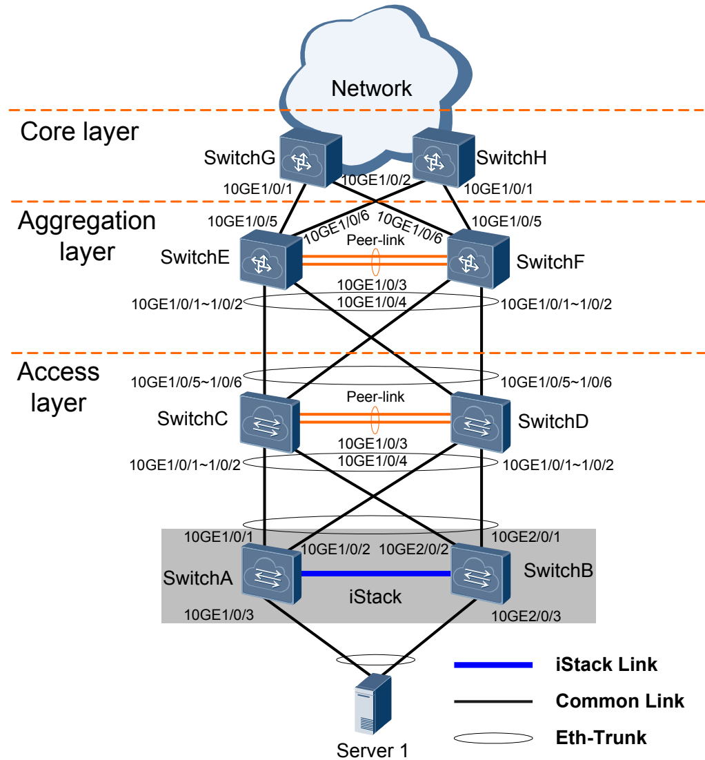
Figure 1-34 Networking for configuring multi-level M-LAG interconnection
