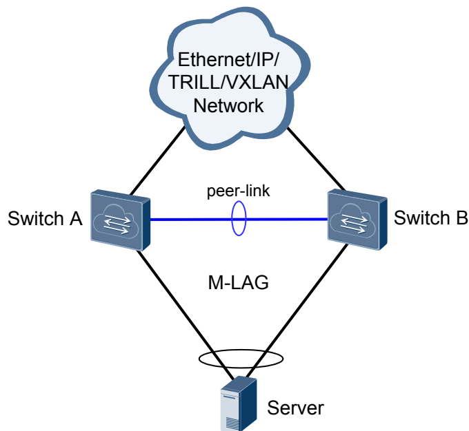
Figure 1-25 Connecting a server in dual-homing mode
