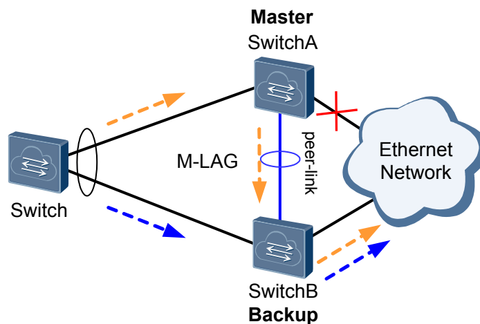
Figure 1-13 Uplink fails
