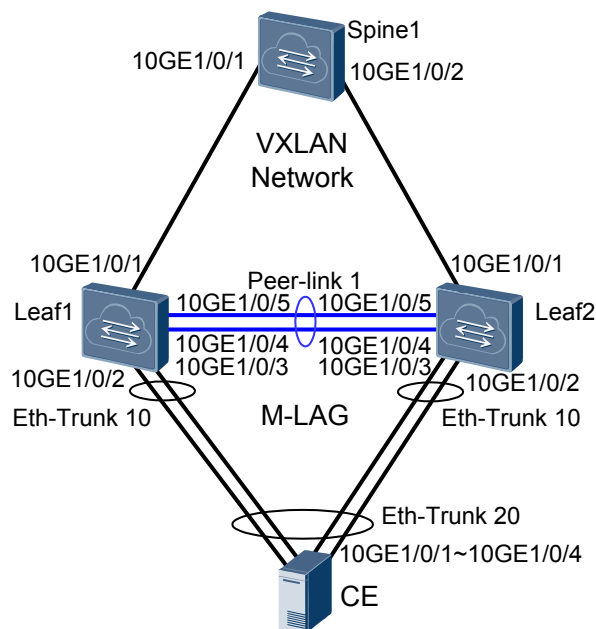
Figure 1-33 VXLAN dual-active access networking
