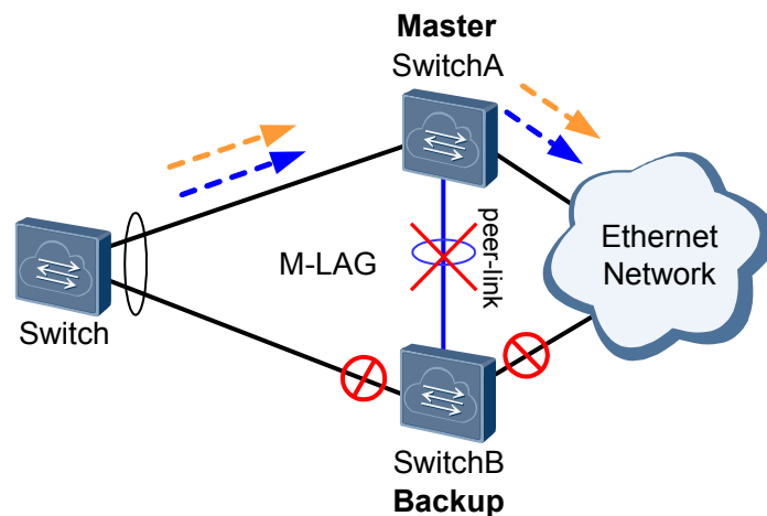
Figure 1-10 Peer-link fails
