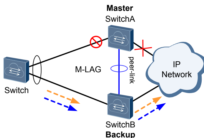
Figure 1-23 Uplink fails
