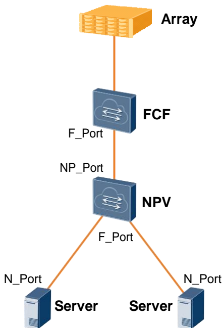
Figure 3-7 NPV networking
