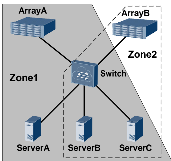
Figure 3-8 Networking of zones
