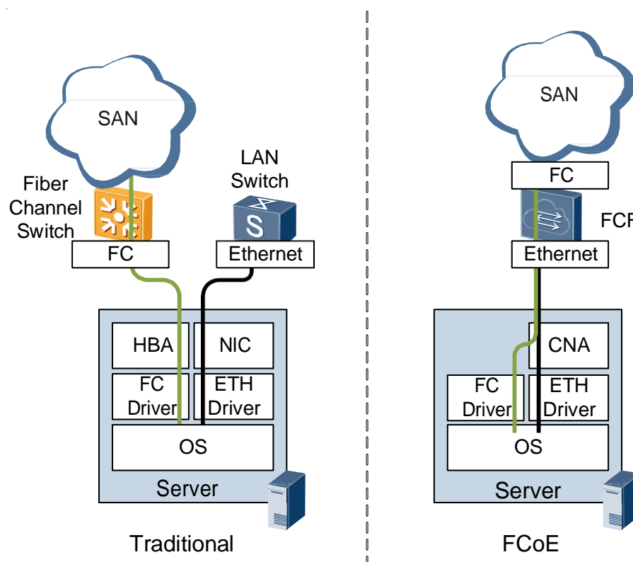
Figure 4-2 Difference between a traditional server and FCoE server
