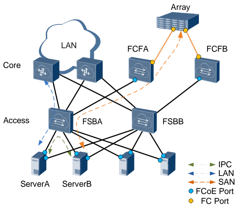
Figure 5-7 Typical FCF+FSB networking (FC interface and FCoE interface)
