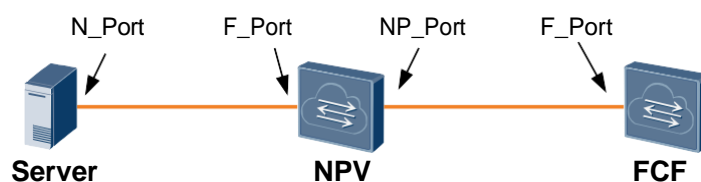
Figure 3-4 Interface role
