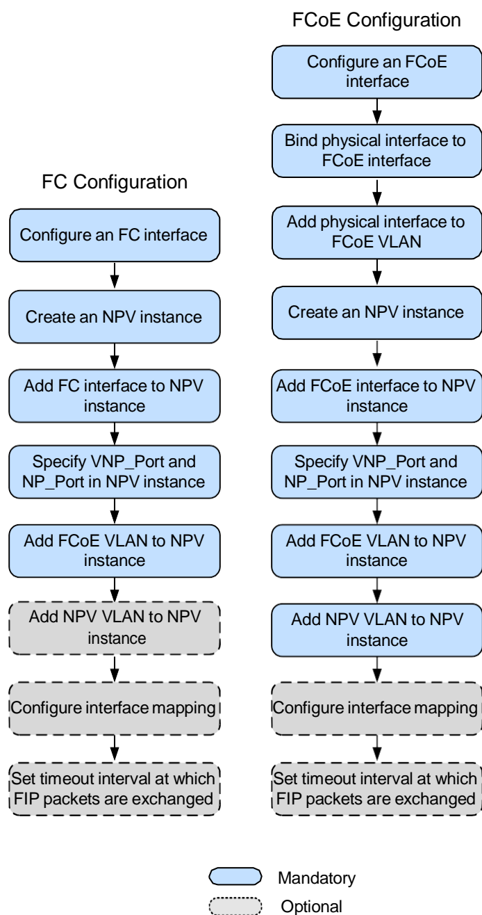
Figure 11-1 NPV configuration flowchart
