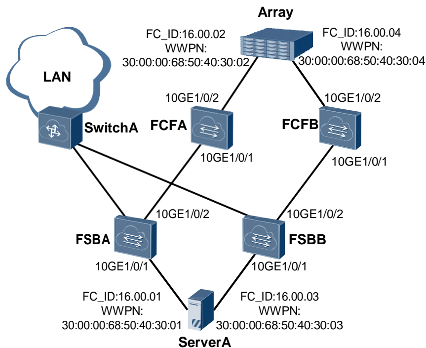
Figure 14-6 Networking of the FCF and FSB
