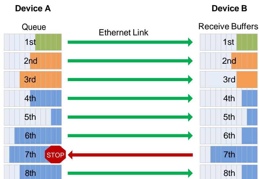
Figure 16-1 PFC working mechanism
