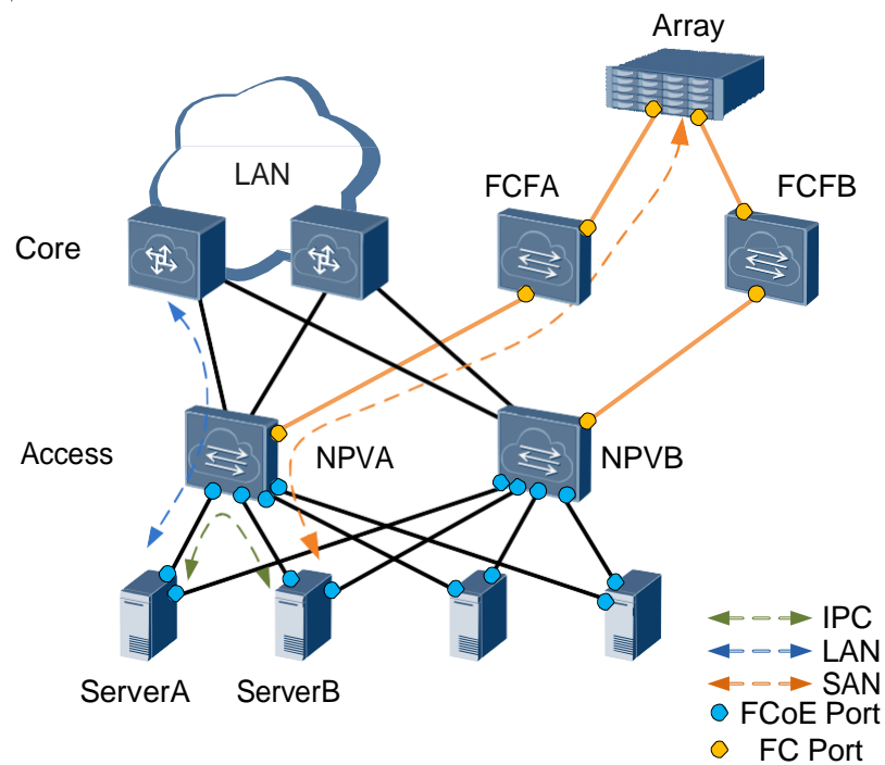
Figure 5-5 Typical networking of the FCF and NPV switch (FC interface and FCoE interface)
