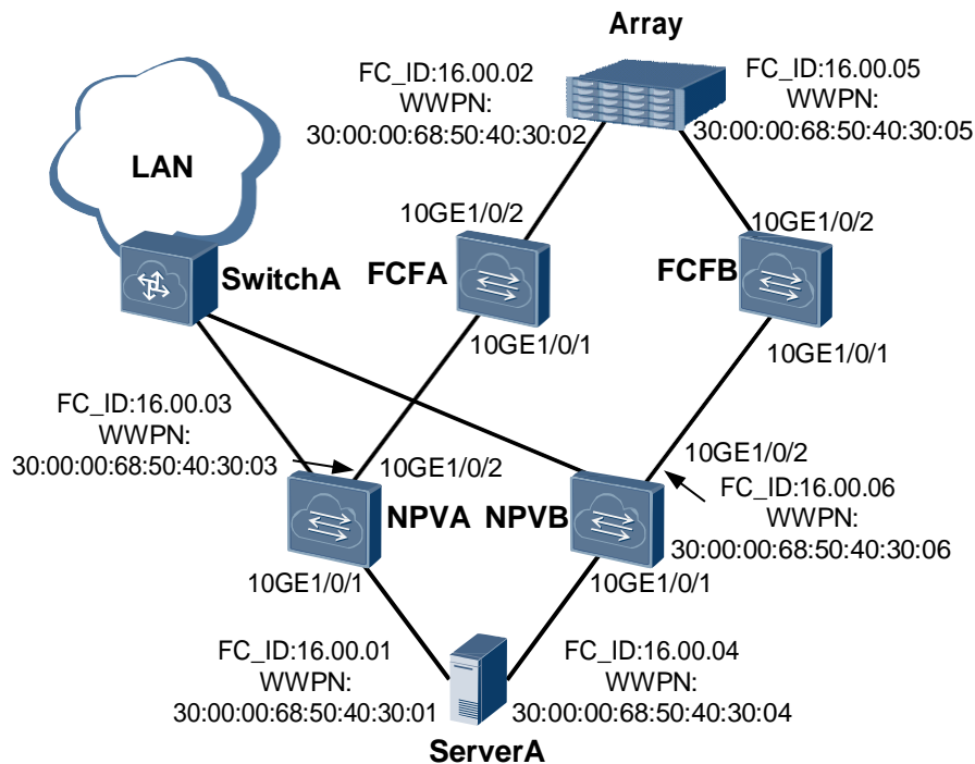
Figure 14-4 Networking of an FCF and an NPV switch
