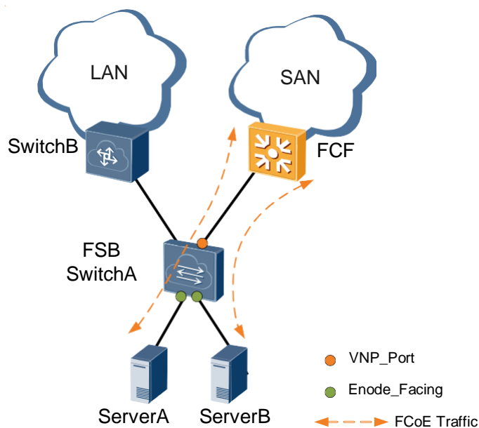
Figure 12-2 Roles of FSB interfaces
