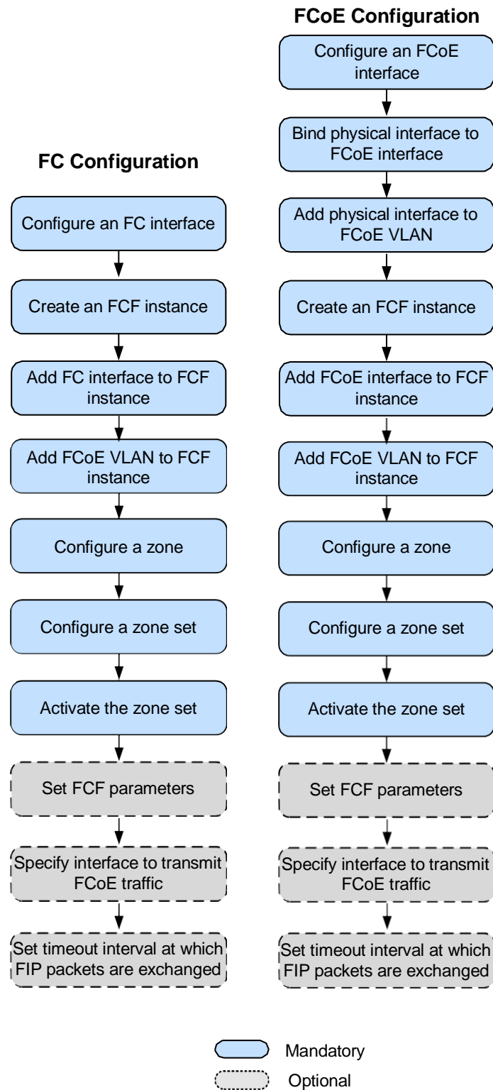
Figure 10-1 FCF configuration flowchart
