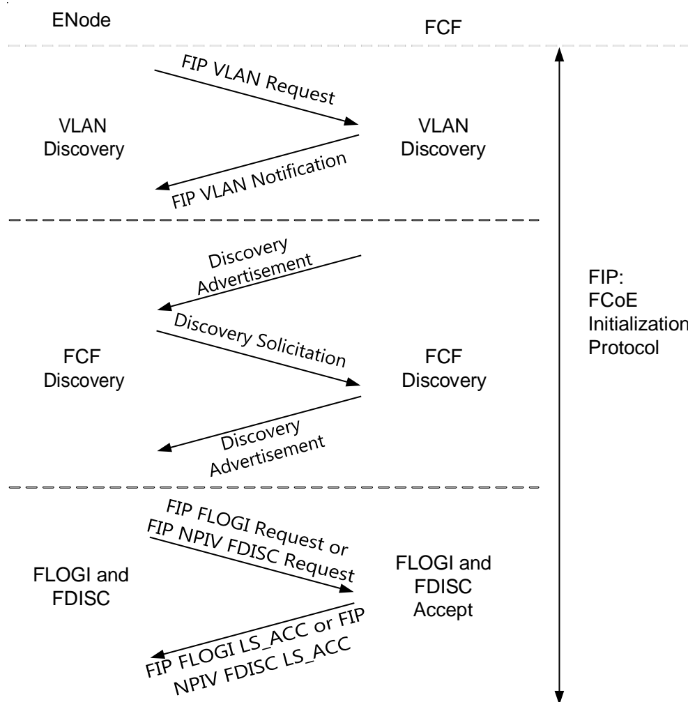
Figure 4-6 FCoE virtual link setup
