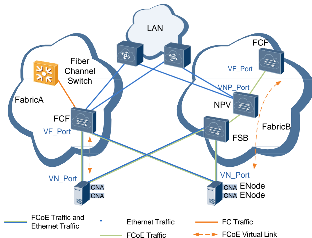
Figure 4-1 FCoE networking
