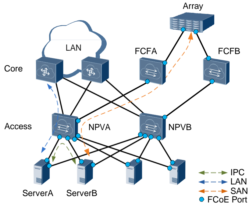
Figure 5-4 Typical networking of the FCF and NPV switch (FCoE interface)
