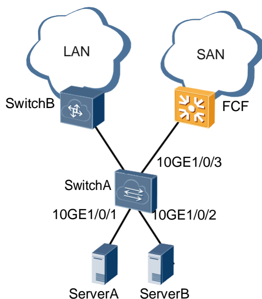
Figure 25-1 Data center networking
