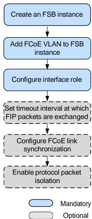
Figure 12-1 FSB configuration flowchart
