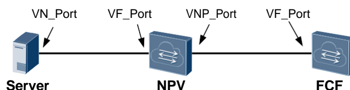
Figure 4-3 Interface roles
