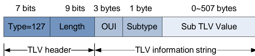
Figure 16-6 DCBX TLV format
