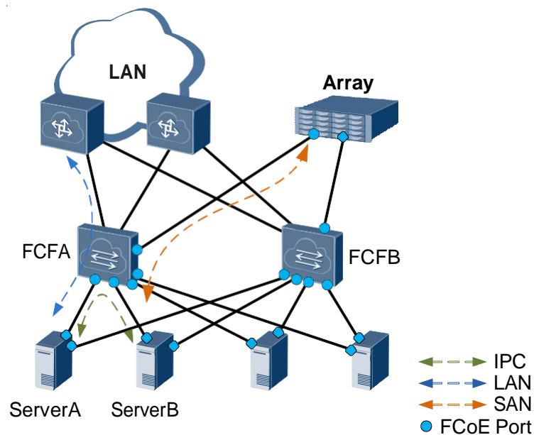
Figure 5-1 Typical FCF networking
