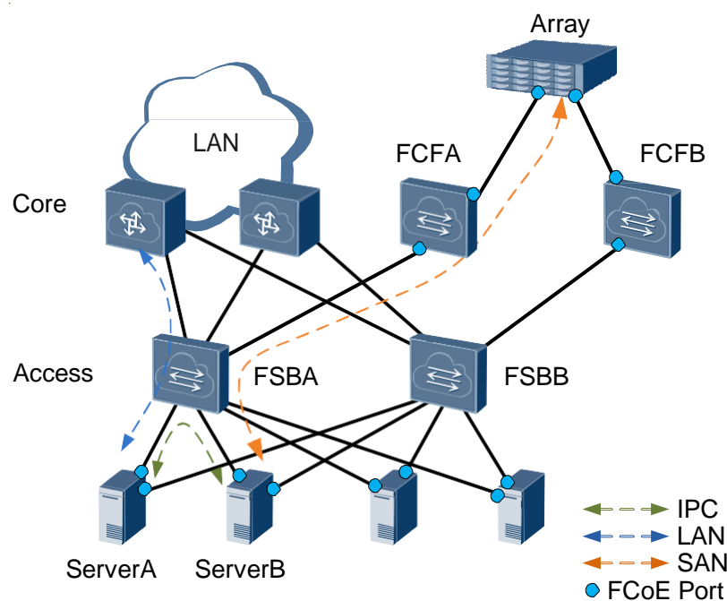
Figure 5-6 Typical FCF+FSB networking (FCoE interface)
