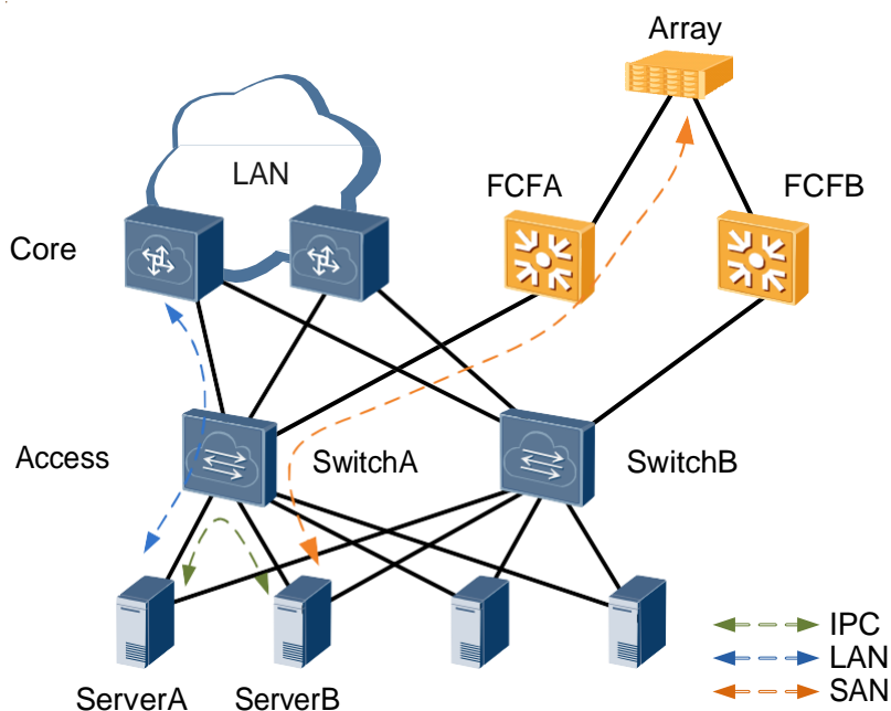
Figure 17-1 FSB networking
