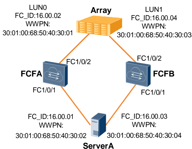
Figure 14-1 FCF networking
