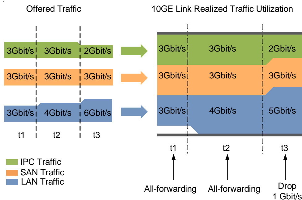
Figure 16-4 Congestion management based on priority groups
