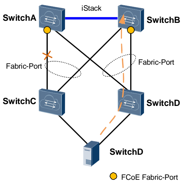
Figure 10-3 SVF networking
