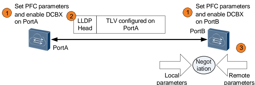
Figure 16-5 DCBX implementation through LLDP
