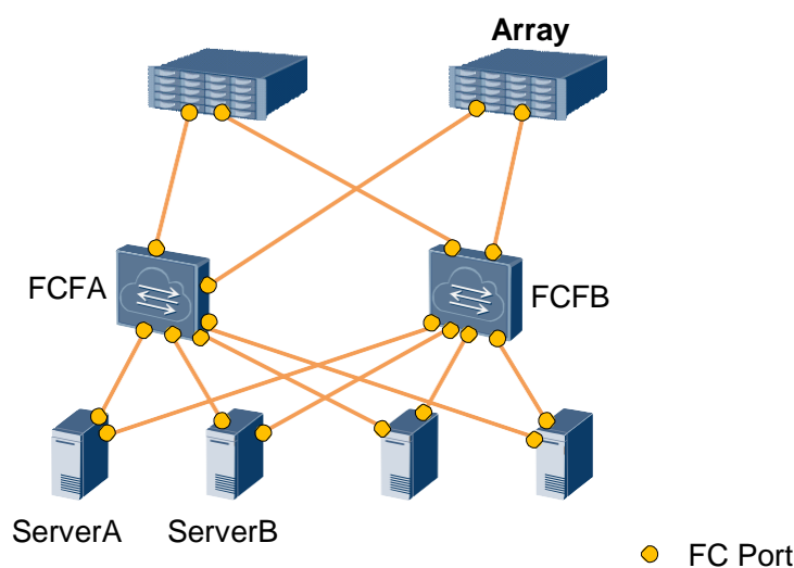
Figure 5-3 Typical FCF networking (FC interface)
