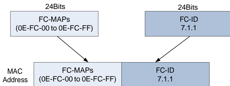
Figure 4-7 FPMA format
