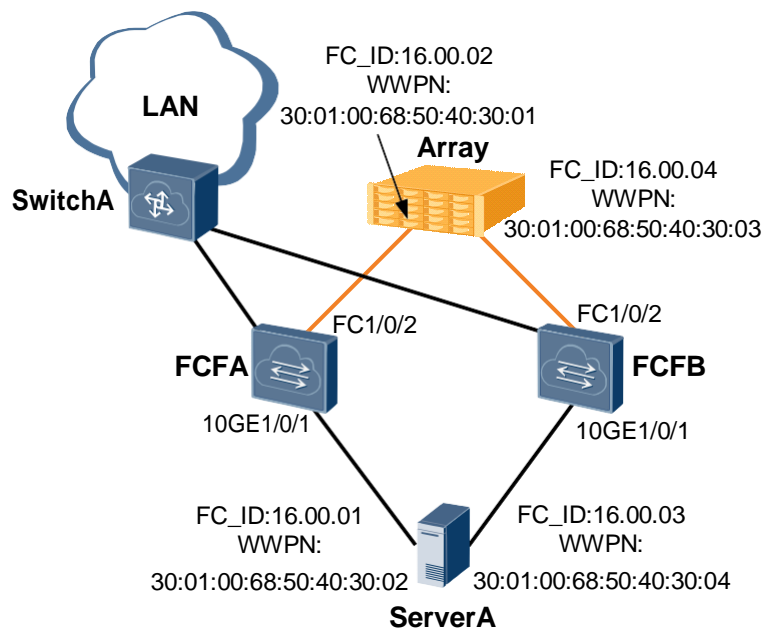
Figure 14-3 FCF networking
