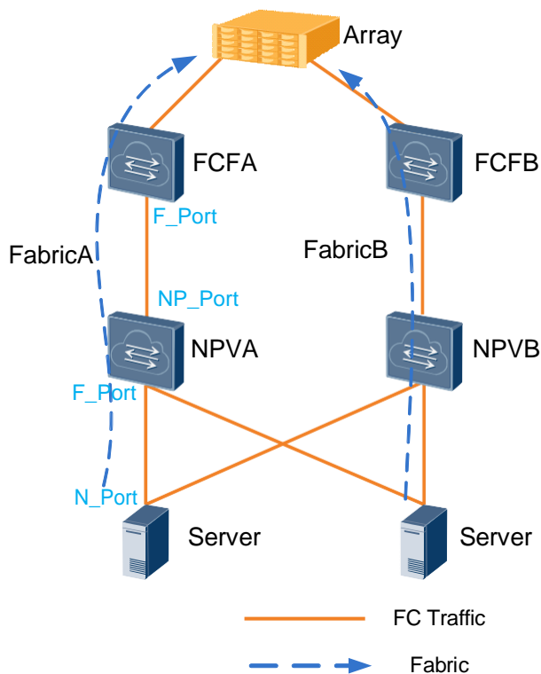
Figure 3-1 FC networking
