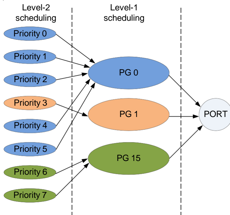
Figure 16-3 ETS Process
