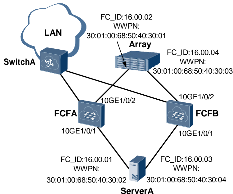
Figure 14-2 FCF networking
