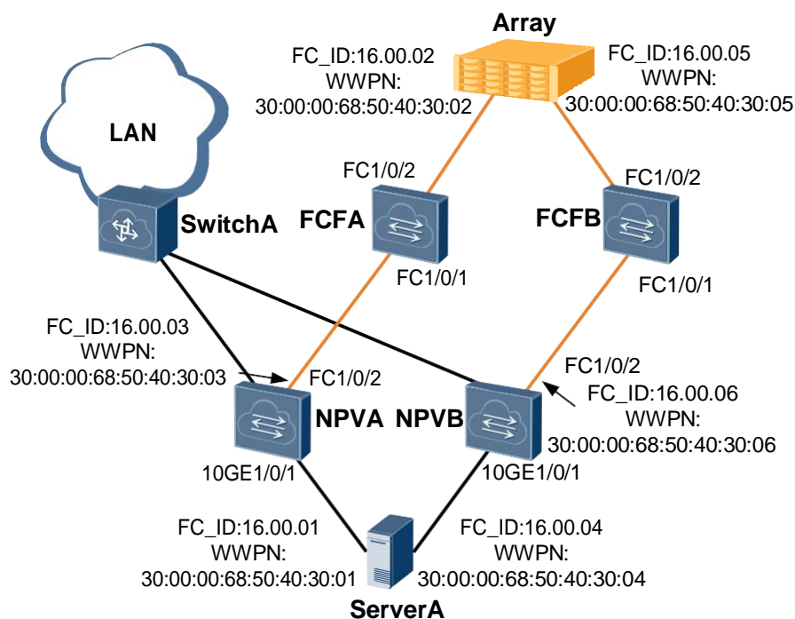
Figure 14-5 FCF+NPV Networking
