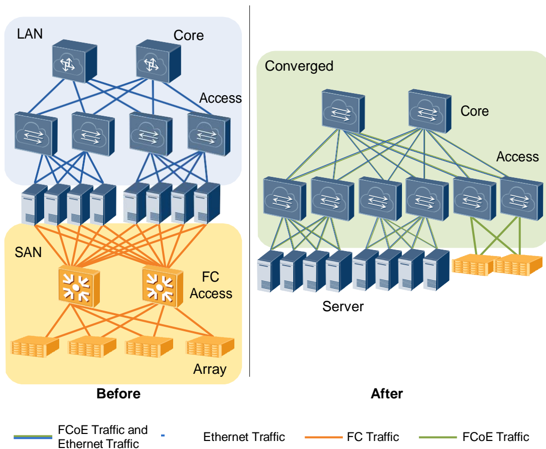
Figure 2-1 Before and after data center network convergence
