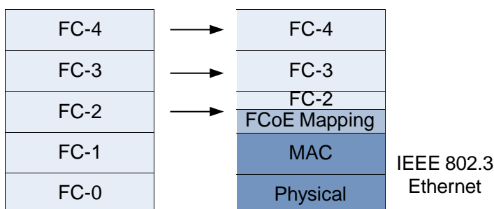
Figure 4-4 Mapping from FC to FCoE
