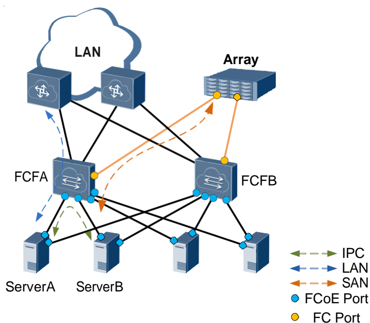
Figure 5-2 Typical FCF networking (FC interface and FCoE interface)
