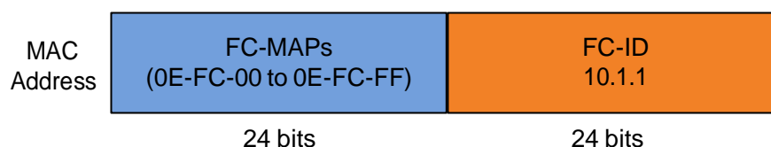
Figure 3-3 FPMA
