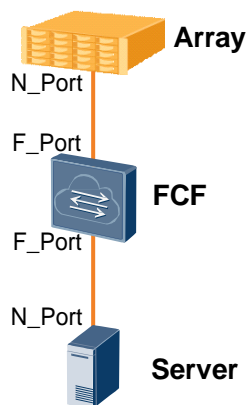
Figure 3-6 FCF networking
