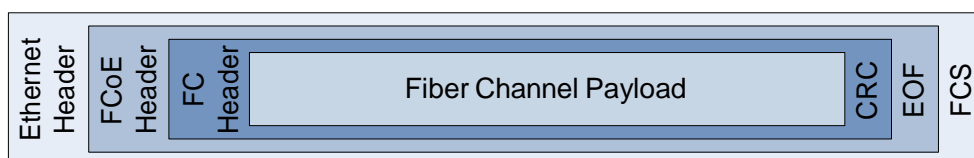
Figure 4-5 FCoE frame encapsulation
