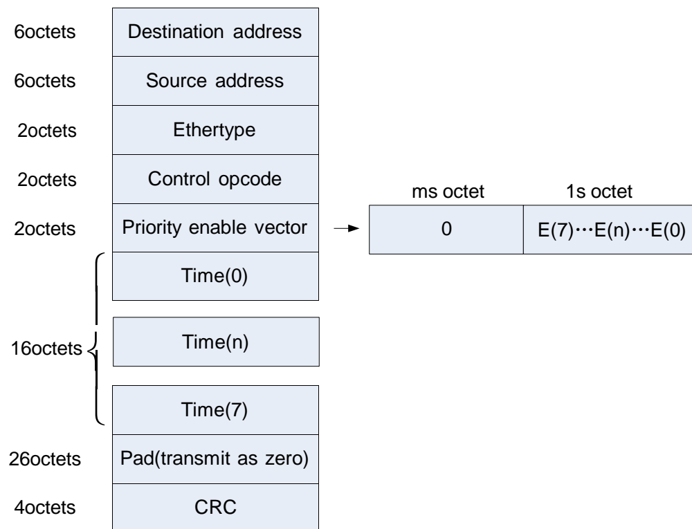
Figure 16-2 PFC frame format
