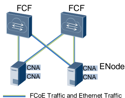
Figure 4-8 Direct connection
