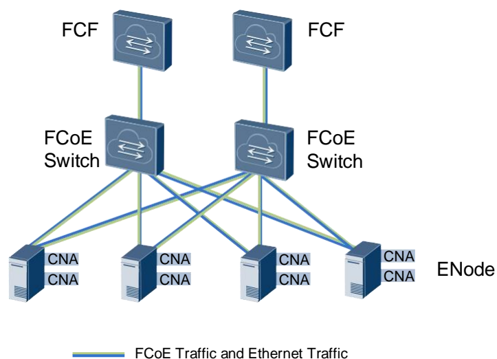
Figure 4-9 Remote connection
