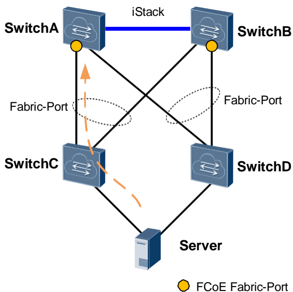
Figure 10-2 SVF networking
