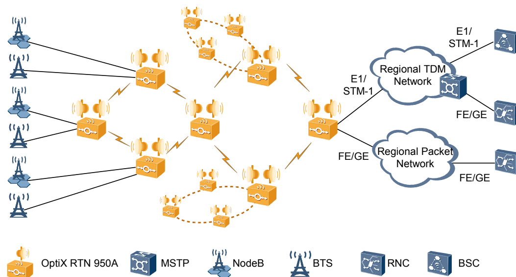
Figure 1-1 Microwave transmission solution provided by the OptiX RTN 950A
