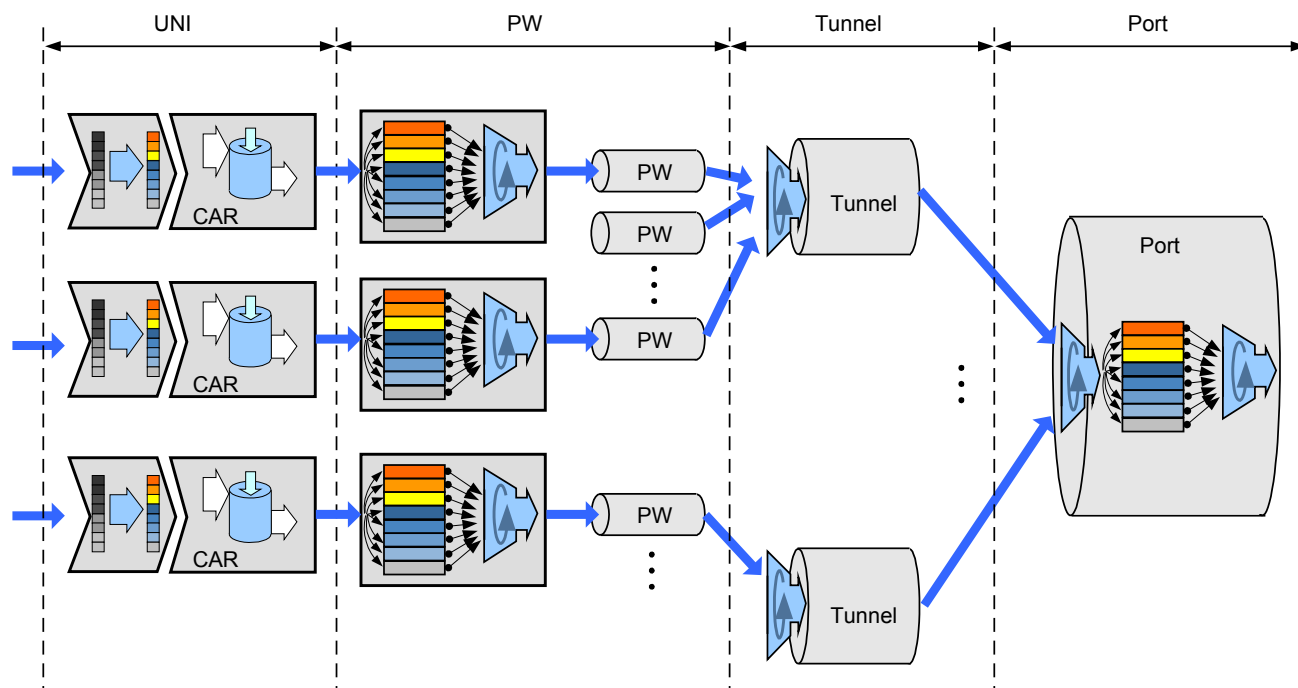
Figure 2-7 Typical HQoS application (ETH PWE3 services)
