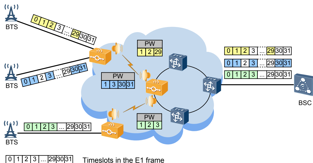
Figure 4-5 Compression of idle 64 kbit/s timeslots in TDM E1 signals
