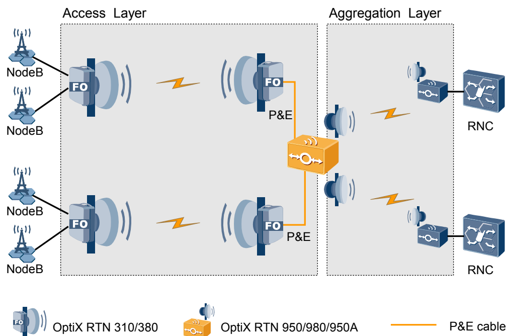
Figure 4-3 Networking with the OptiX RTN 310/380
