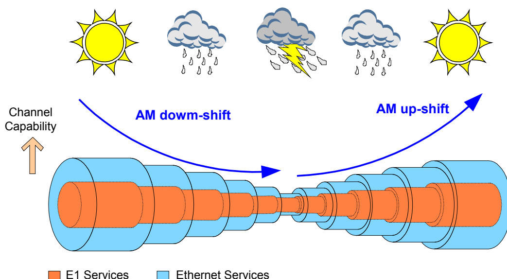
Figure 2-3 Adaptive modulation
