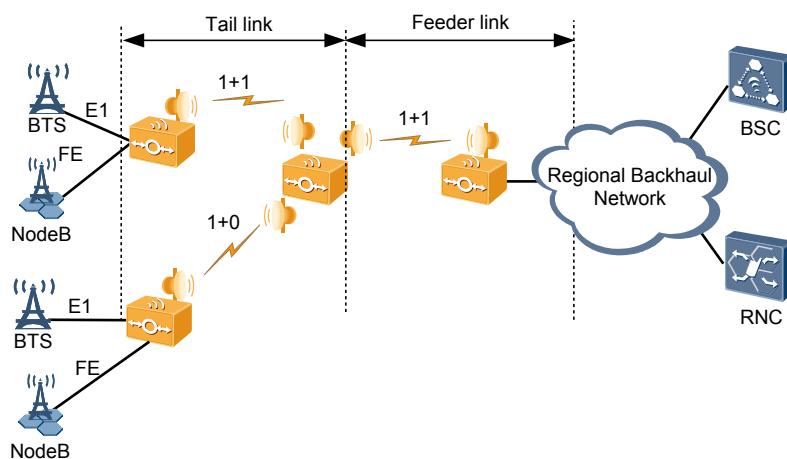
Figure 4-1 Radio transmission solution based on chain networks
