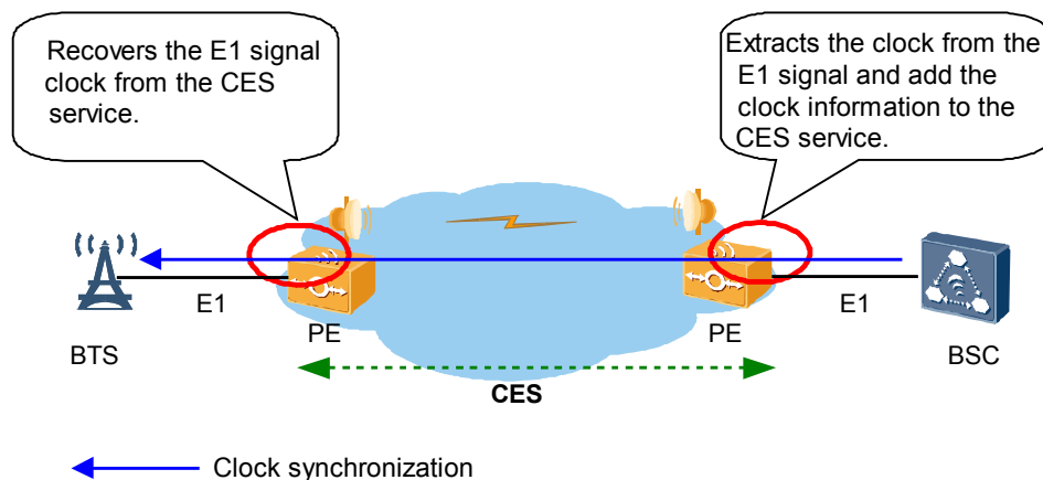
Figure 4-7 Adaptive synchronization mode of CES service clocks
