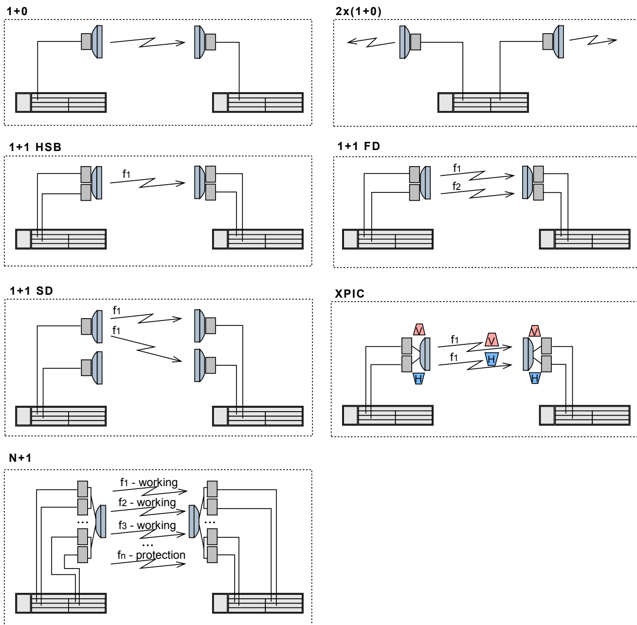
Figure A-1 Typical RF configuration modes
