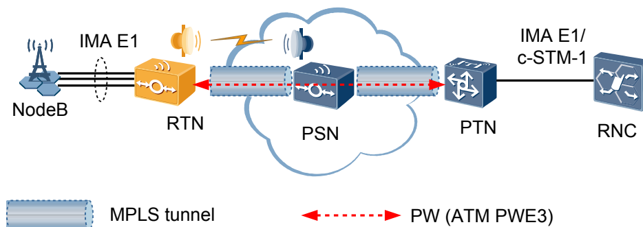
Figure 4-9 Example of ATM/IMA services
