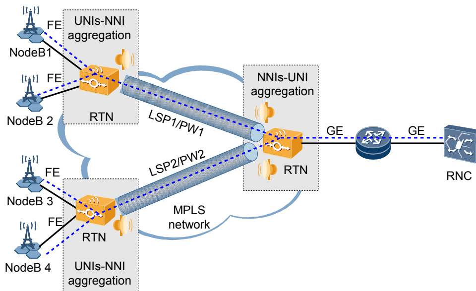
Figure 4-11 Example of E-Aggr services
