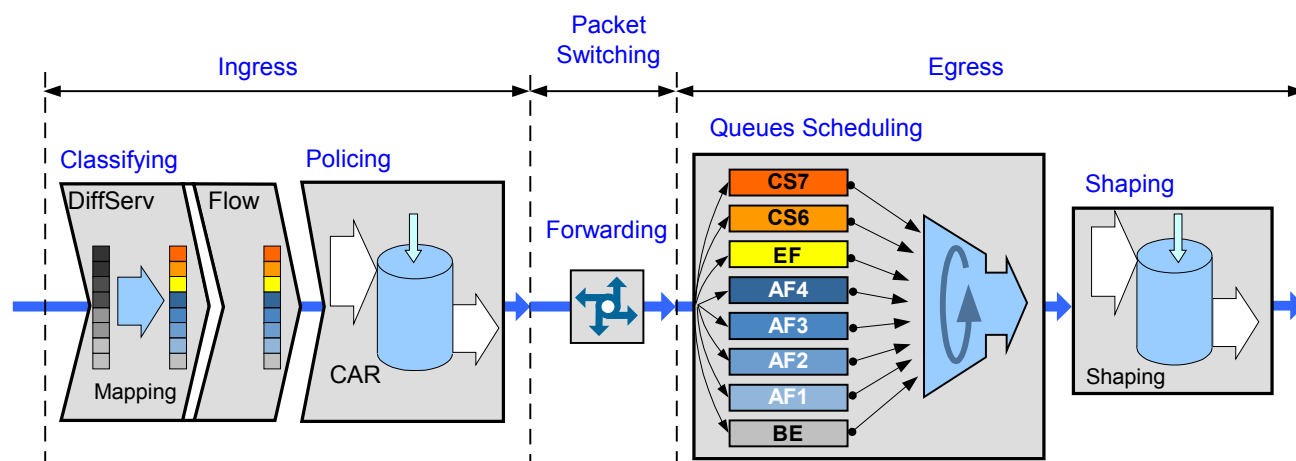
Figure 2-6 Typical QoS application (Native Ethernet services)
