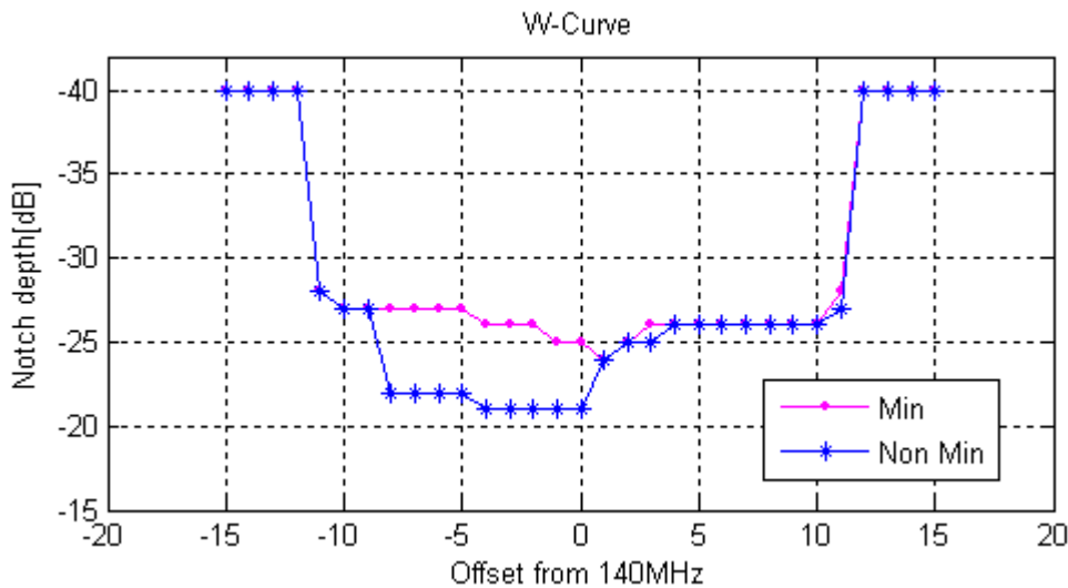
Figure 6-2 W-curve
