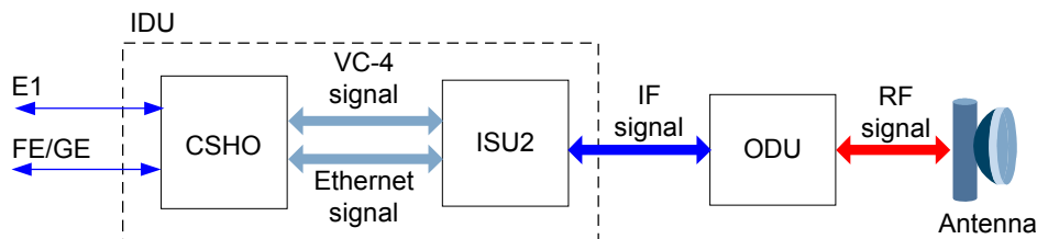
Figure 3-6 Service signal processing flow of the Hybrid microwave
