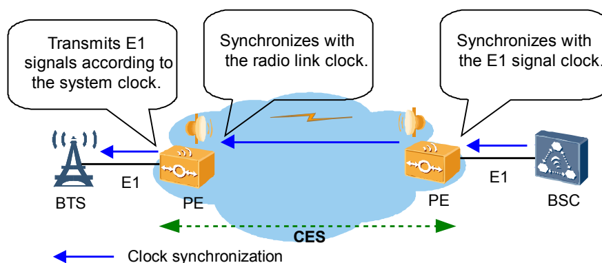
Figure 4-6 Retiming synchronization mode of CES service clocks
