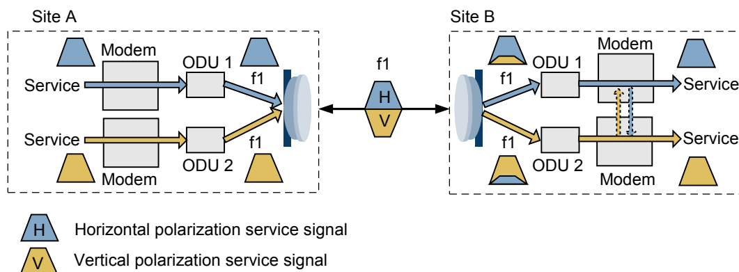
Figure 2-4 CCDP channel configuration and XPIC technology
