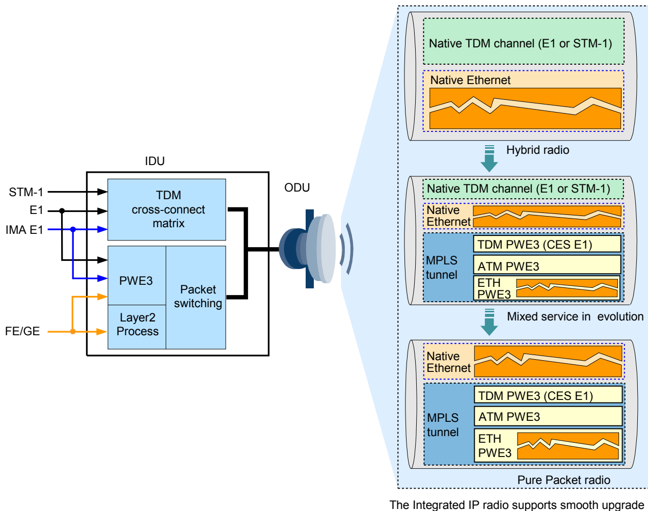
Figure 2-2 Hybrid/Packet integrated IP microwave
