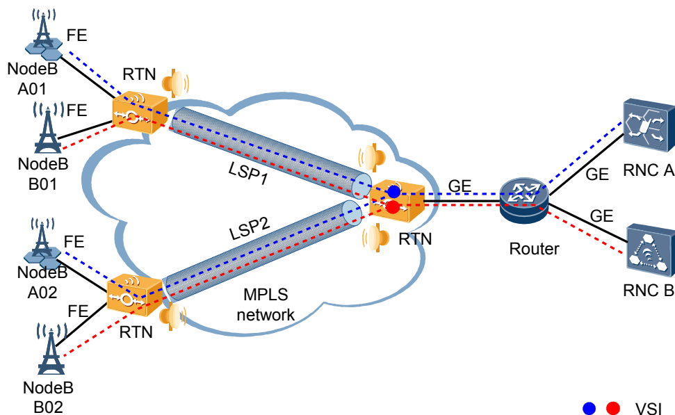
Figure 4-12 Example of VPLS services
