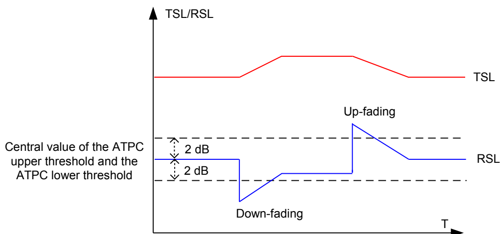
Figure 2-5 Relationship between the RSL and TSL
