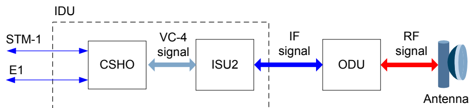
Figure 3-5 Service signal processing flow of the SDH microwave
