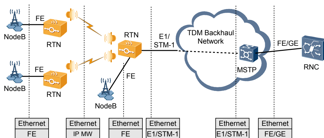
Figure 4-13 Traversing a TDM network using the EoPDH/EoSDH feature
