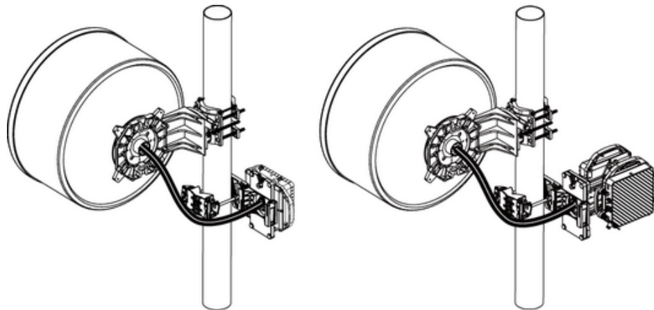
Figure 1-4 Separate mounting
