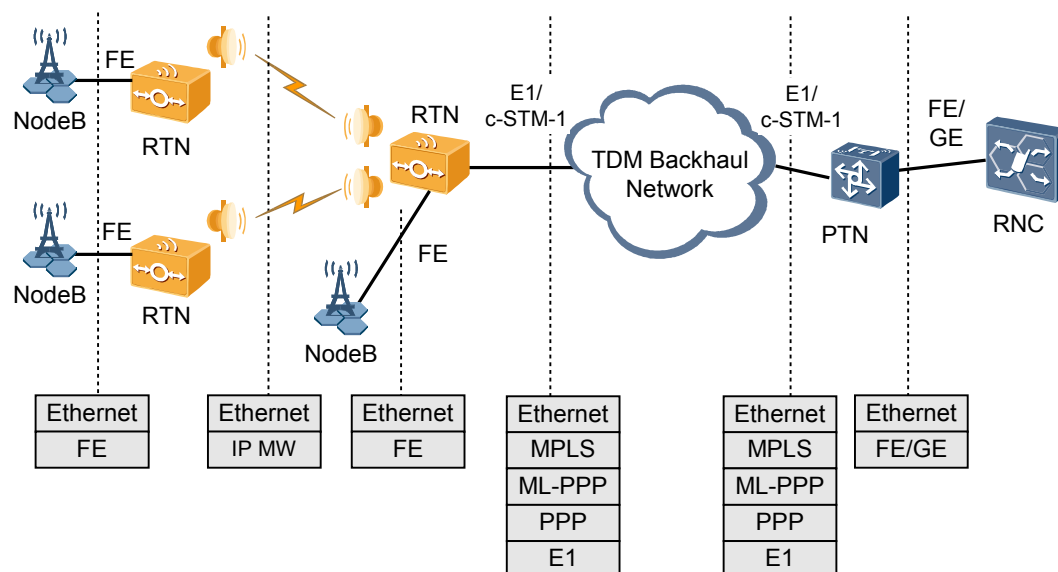
Figure 4-14 Using ML-PPP to transmit services through a TDM network
