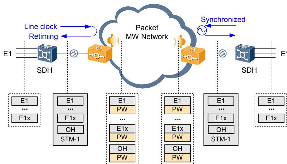
Figure 4-8 Channelized STM-1 emulation
