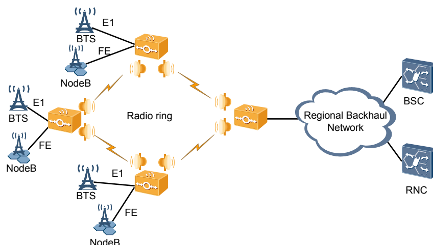
Figure 4-2 Radio transmission solution based on ring networks
