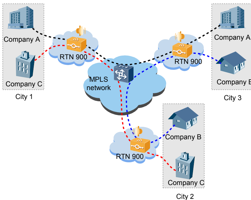
Figure 4-10 Example of E-Line services
