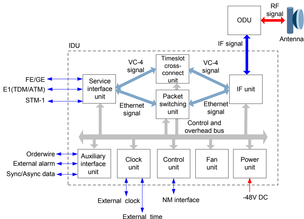
Figure 3-1 Block diagram
