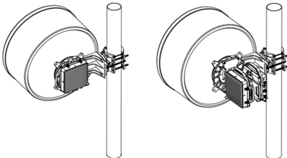
Figure 1-3 Direct mounting
