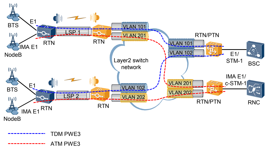
Figure 4-15 MPLS tunnels traversing a Layer 2 network using VLAN sub-interfaces
