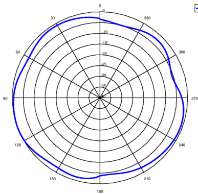
2.4G (PHI=0)
