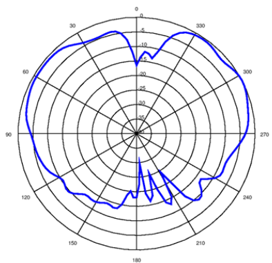
2.4G (PHI=90)
