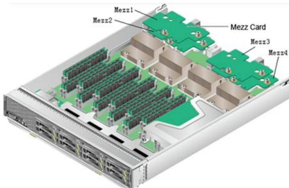
Figure 1-3 MZ310 installation positions on a full-width compute node
