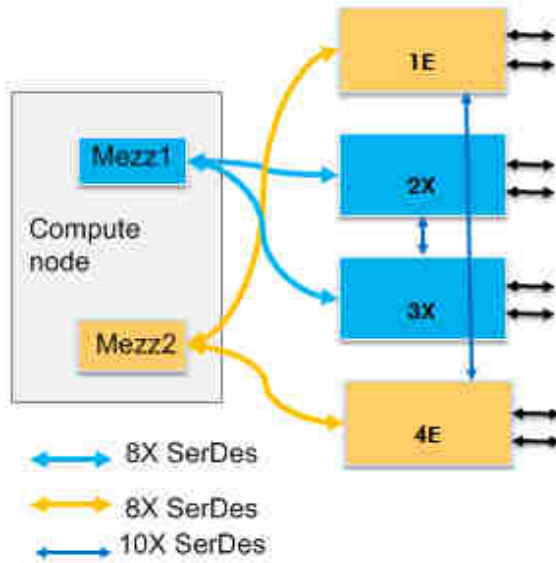
Figure 3-1 Connections between the MZ310s on a half-width compute node and the ports on I/O modules
