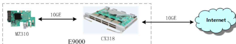
Figure 3-5 Connection between the MZ310 and the CX318
