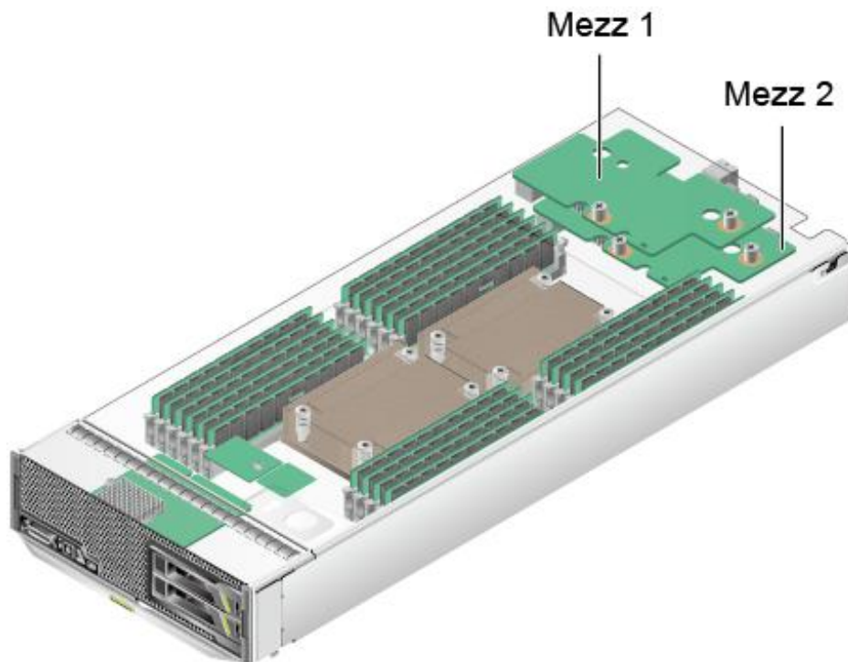
Figure 1-2 MZ310 installation positions on a half-width compute node
