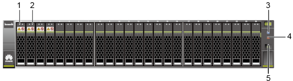
Figure 4-20 Indicators on the front panel of a 2 U 25-disk controller enclosure
