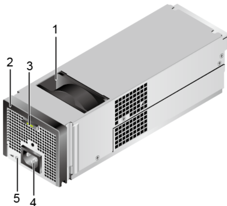
Figure 4-11 Front view of an AC power module
