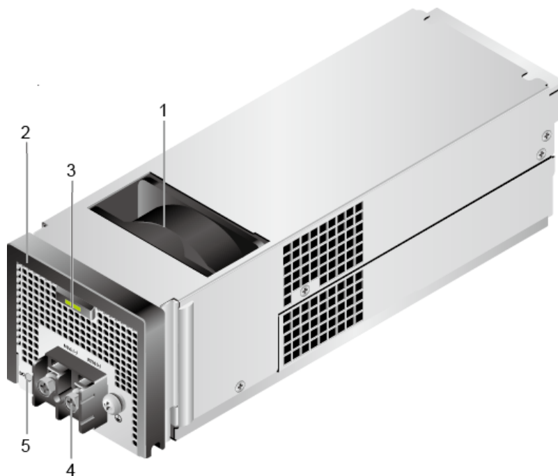
Figure 4-12 Front view of a DC power module
