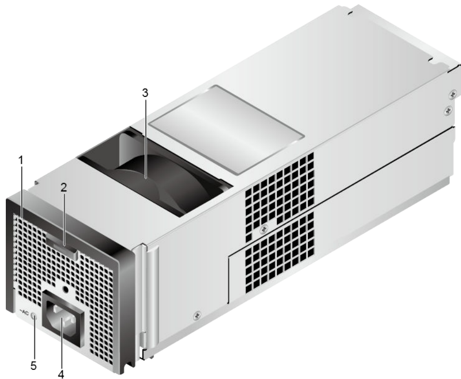
Figure 4-42 AC power module
