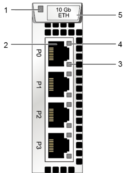
Figure 4-18 10GE electrical interface module
