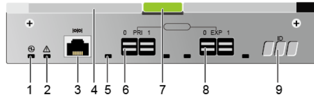
Figure 4-54 Ports on an expansion module
