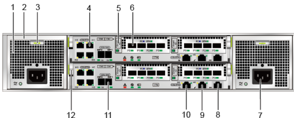
Figure 4-7 Rear view of the OceanStor 2600 V3 controller enclosure (with AC power modules and dual controllers)
