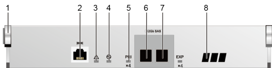
Figure 4-41 Interfaces of an expansion module
