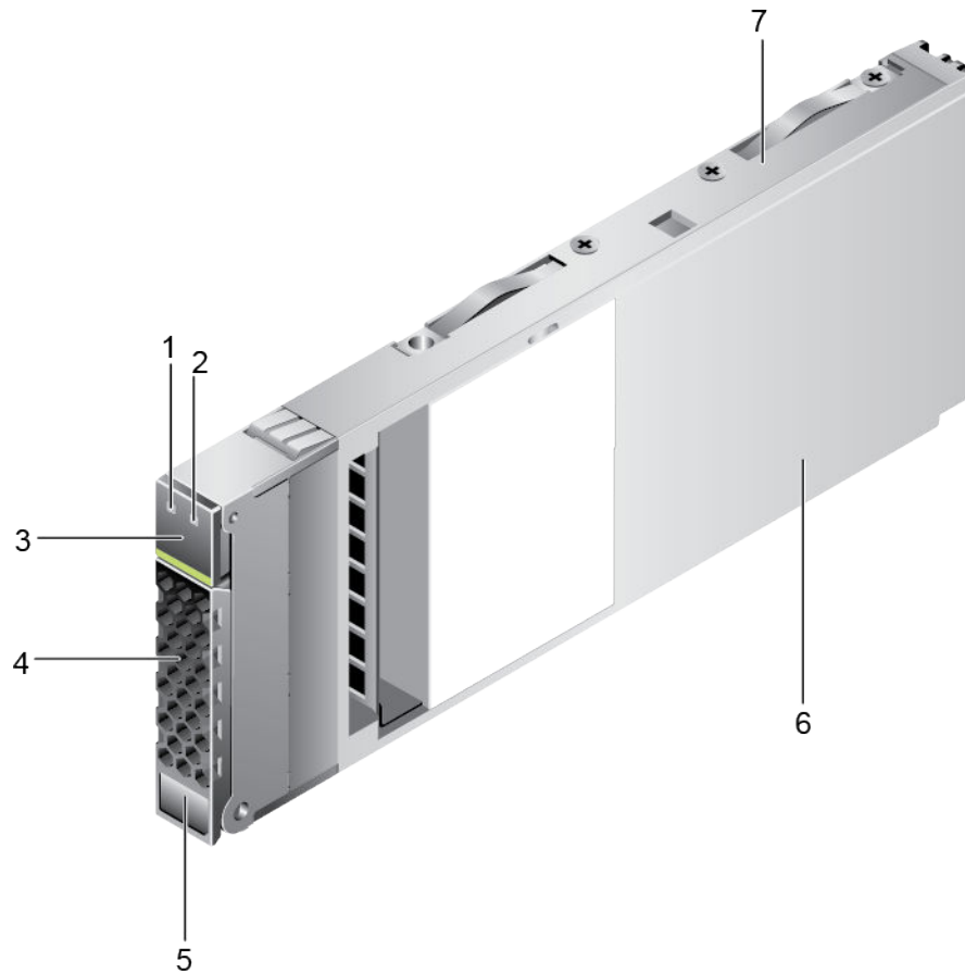
Figure 4-32 Disk module
