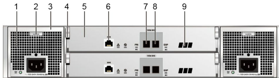
Figure 4-26 Rear view of a disk enclosure with the AC power module
