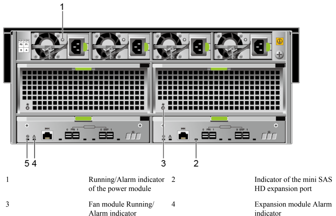
Figure 4-59 Indicators on the rear panel of a high-density disk enclosure
