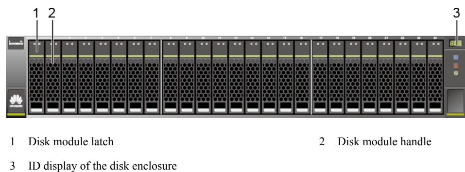
Figure 4-24 Front view of a 2 U disk enclosure
