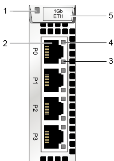
Figure 4-17 GE electrical interface module
