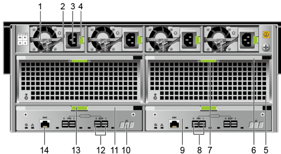
Figure 4-50 Rear view of a high-density disk enclosure
