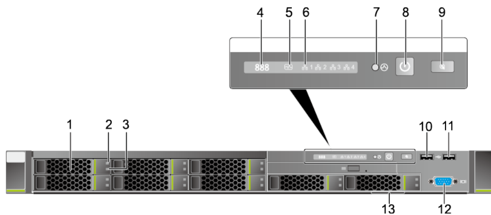
Figure 4-64 Front panel of the quorum server
