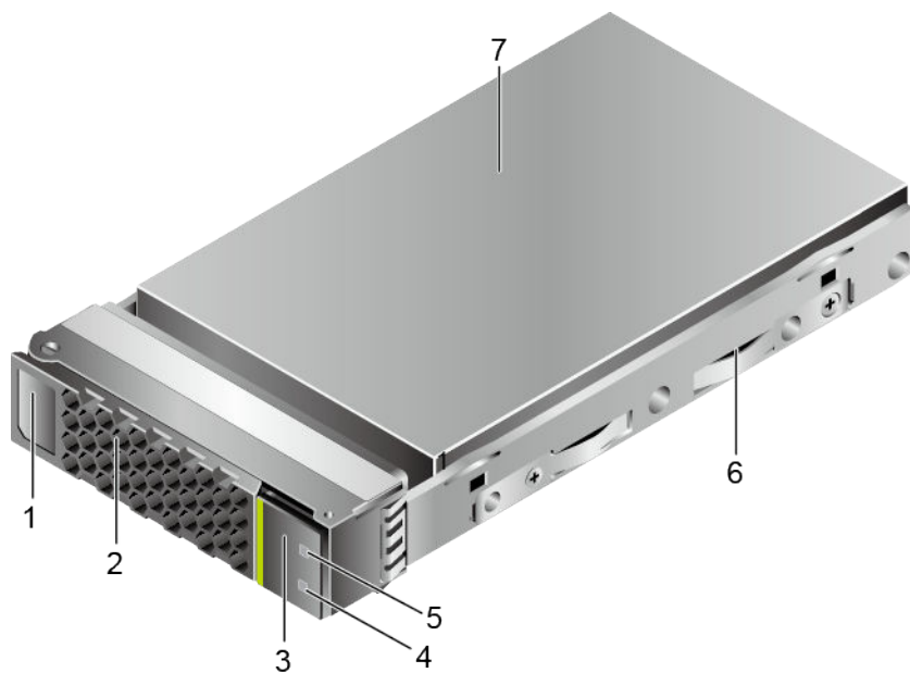
Figure 4-14 3.5-inch disk module
