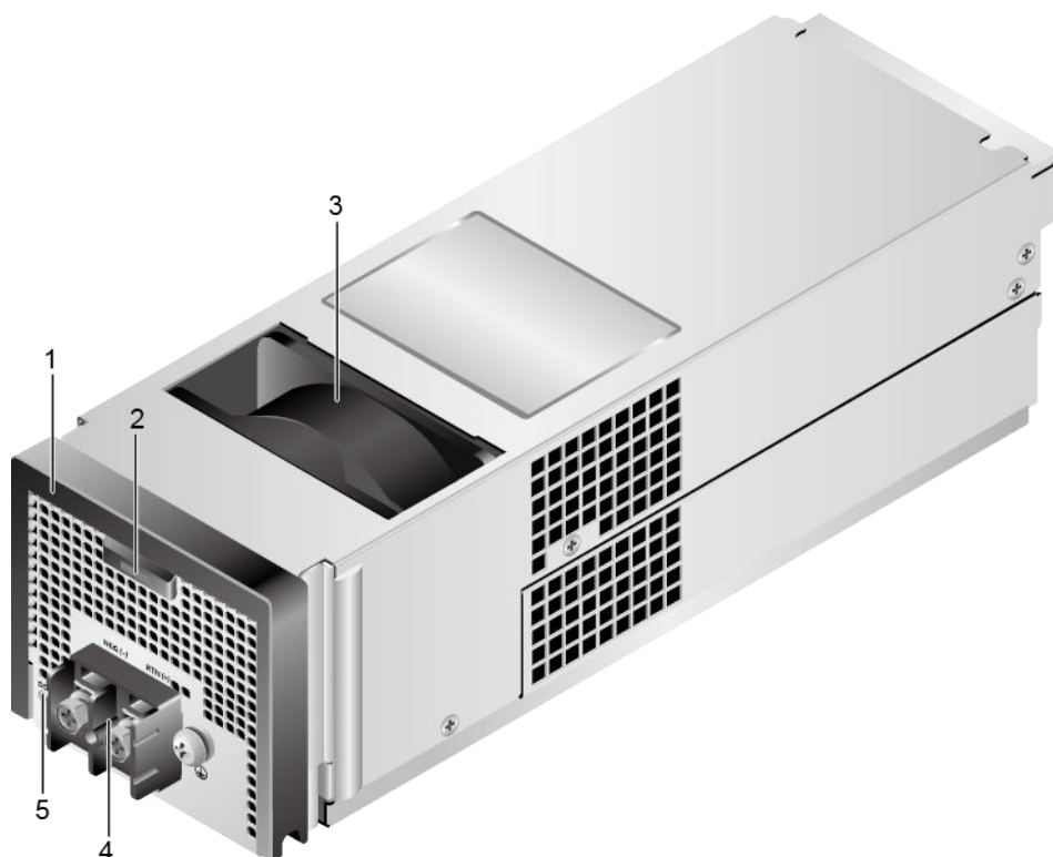
Figure 4-43 DC power module
