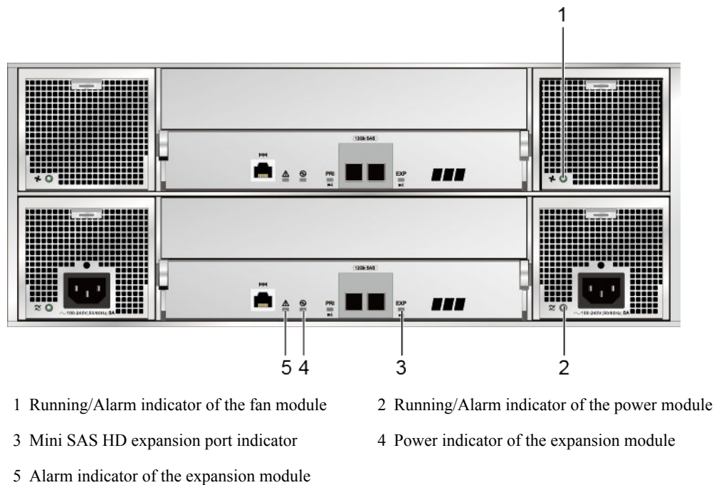
Figure 4-47 Indicators on the rear panel of a disk enclosure
