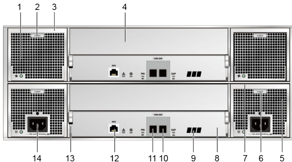
Figure 4-38 Rear view of a disk enclosure with the AC power module
