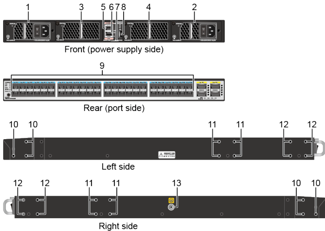
Figure 4-63 Appearance of the data switch
