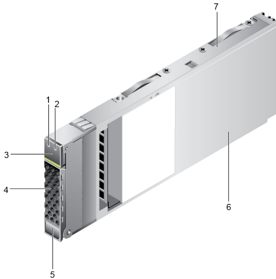
Figure 4-13 2.5-inch disk module
