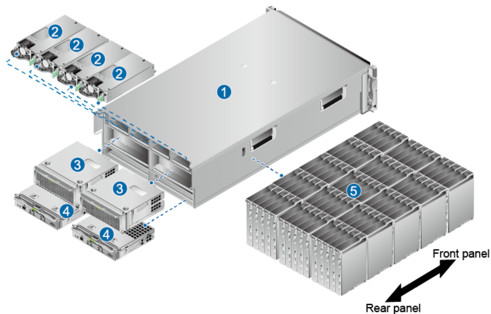
Figure 4-48 Overall structure of a high-density disk enclosure with four 1200 W power modules
