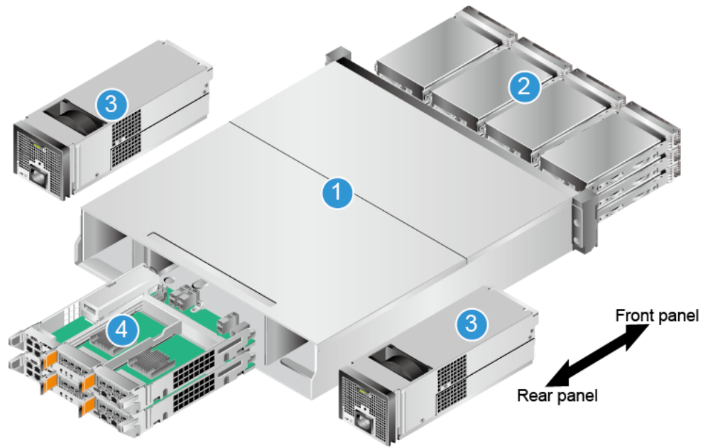
Figure 4-2 Overall structure of a 2 U 12-disk controller enclosure
