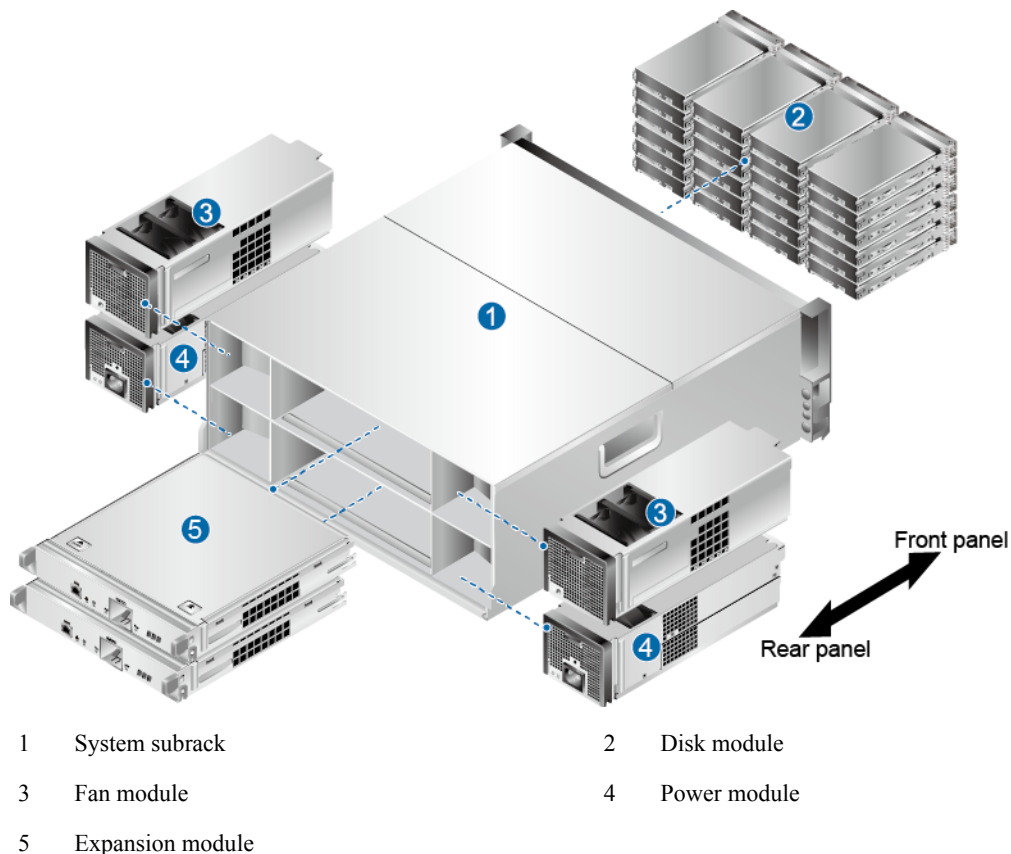
Figure 4-35 Overall structure of a 4 U disk enclosure
