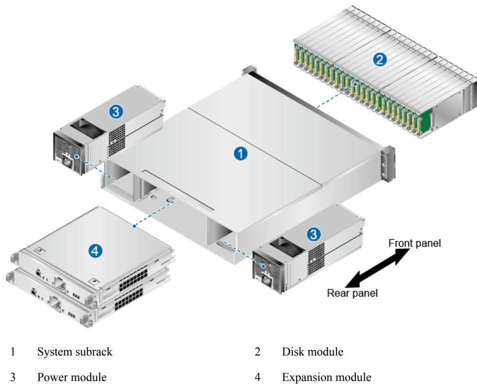
Figure 4-23 Overall structure of a 2 U SAS disk enclosure
