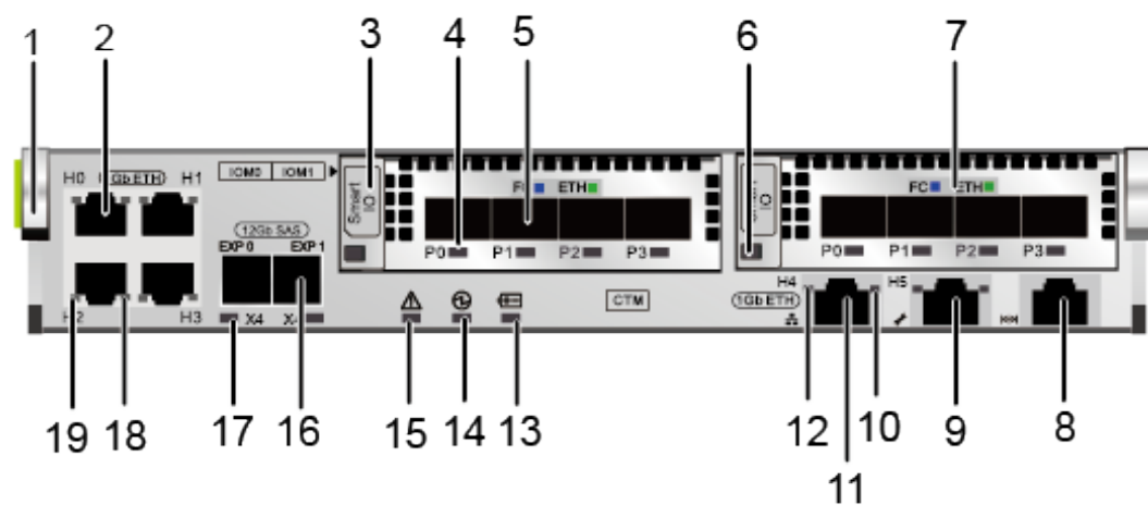
Figure 4-10 Ports of a controller
