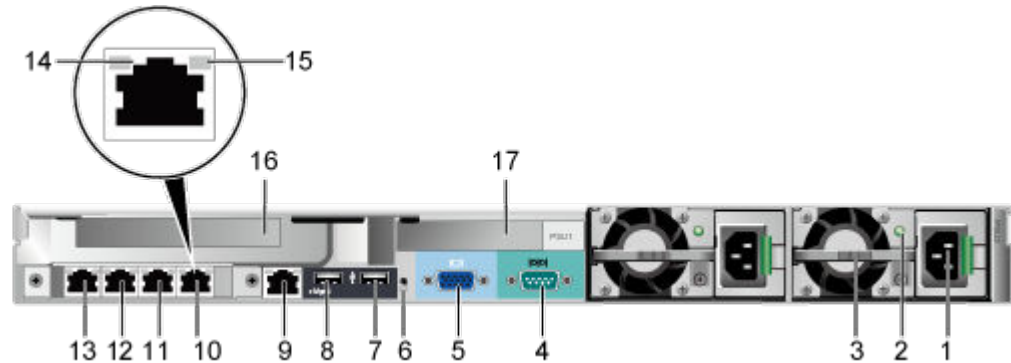
Figure 4-65 Rear view of the quorum server
