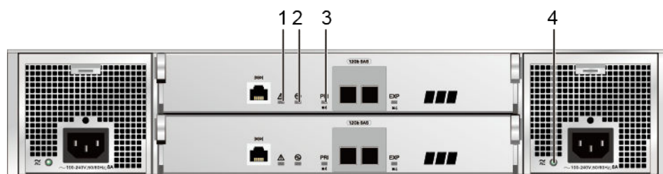
Figure 4-34 Indicators on the rear panel of a disk enclosure
