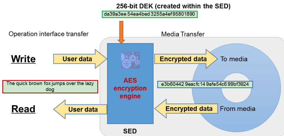
Figure 3-7 Data encryption
