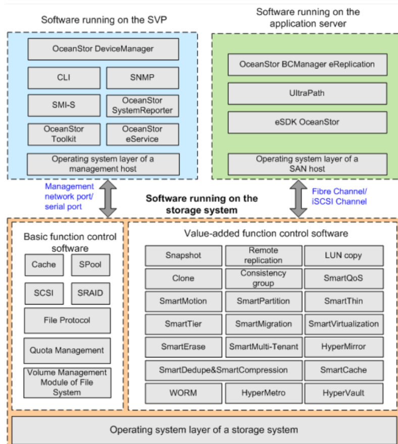
Figure 3-8 Software architecture
