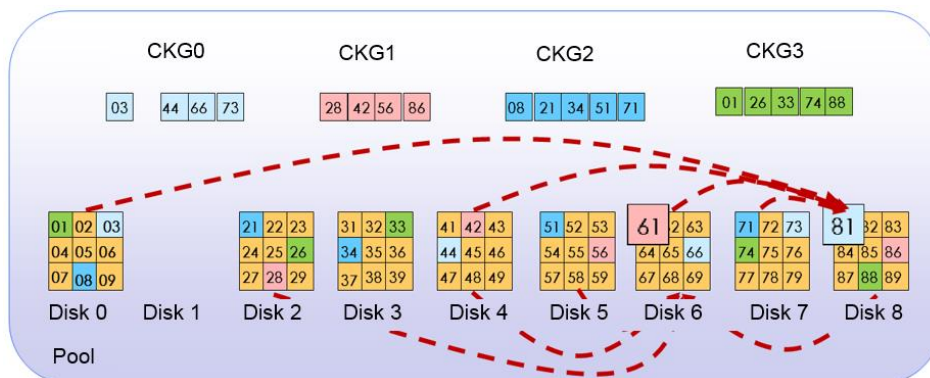
Figure 3-11 RAID 2.0+ fast reconstruction (2)
