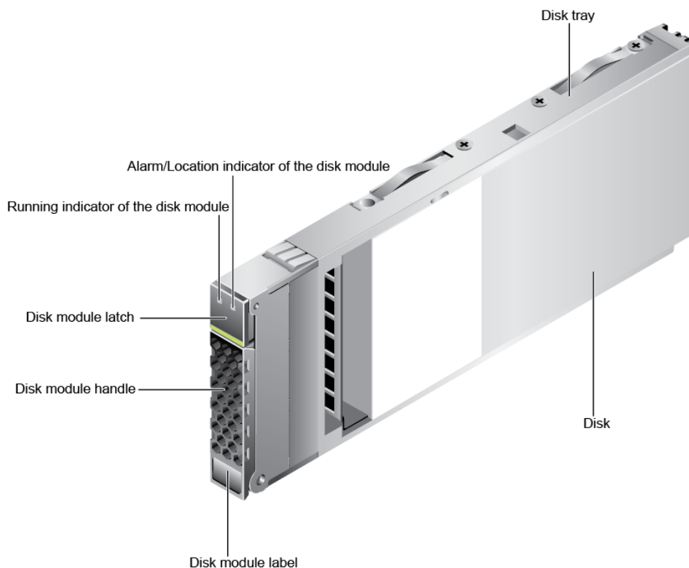
Figure 4-59 Disk module
