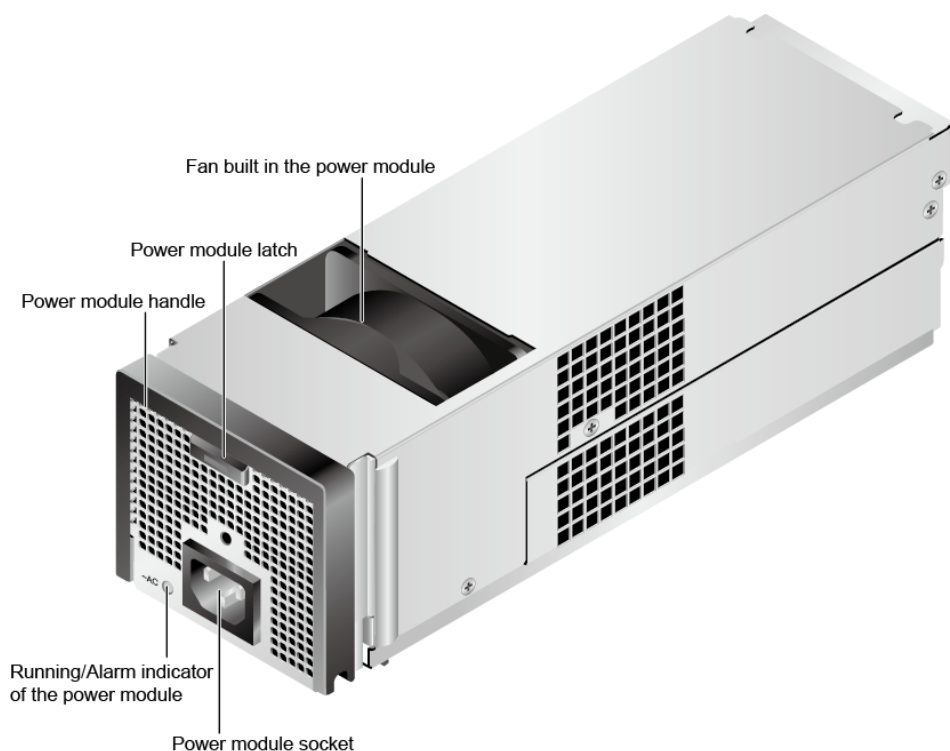
Figure 4-58 AC power module
