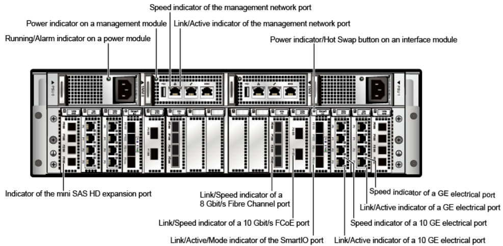
Figure 4-25 Indicators on the rear panel of a controller enclosure
