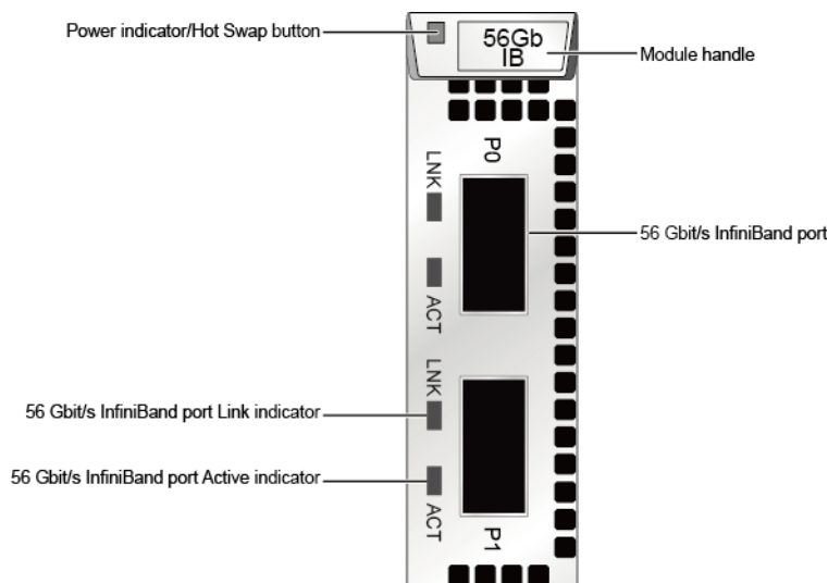
Figure 4-48 56 Gbit/s IB interface module
