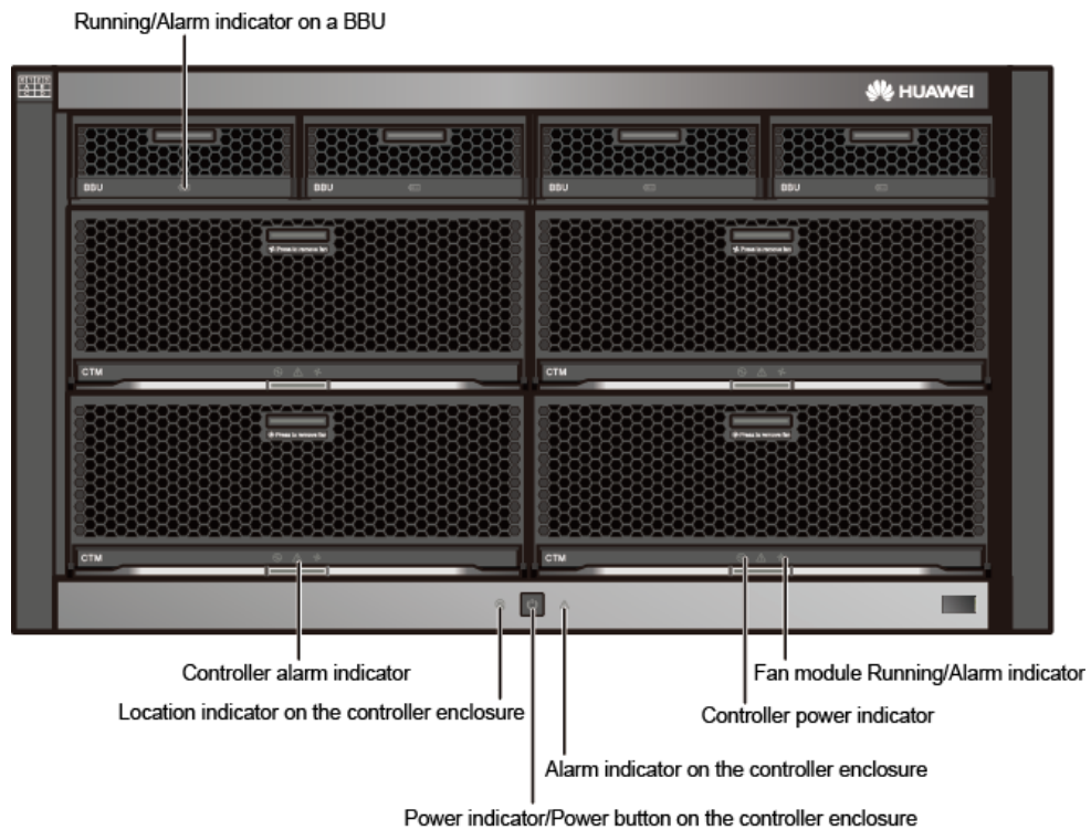
Figure 4-40 Indicators on the front panel of a controller enclosure
