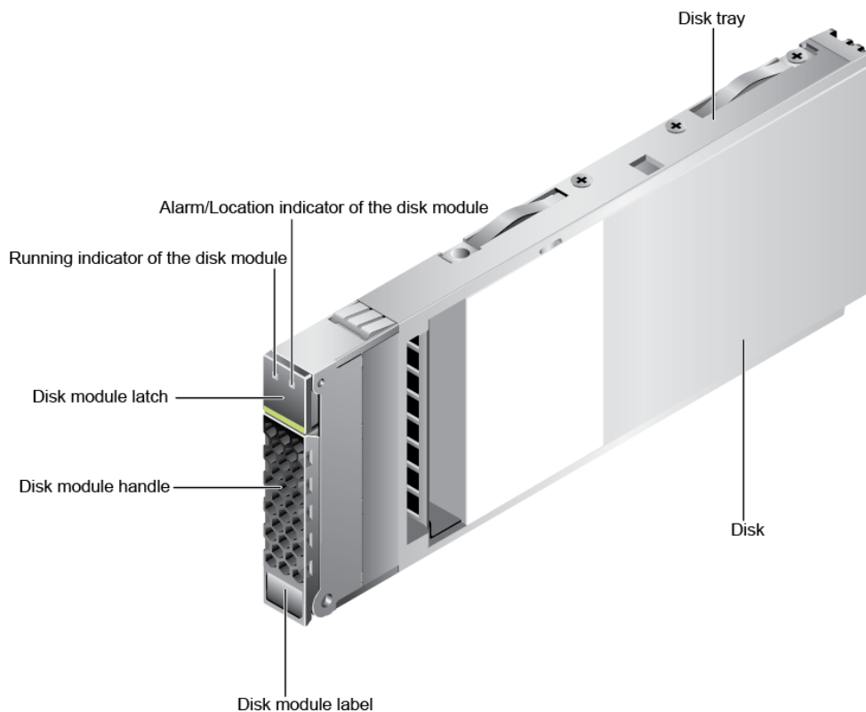
Figure 4-9 Disk module
