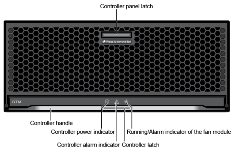
Figure 4-17 Front view of a controller
