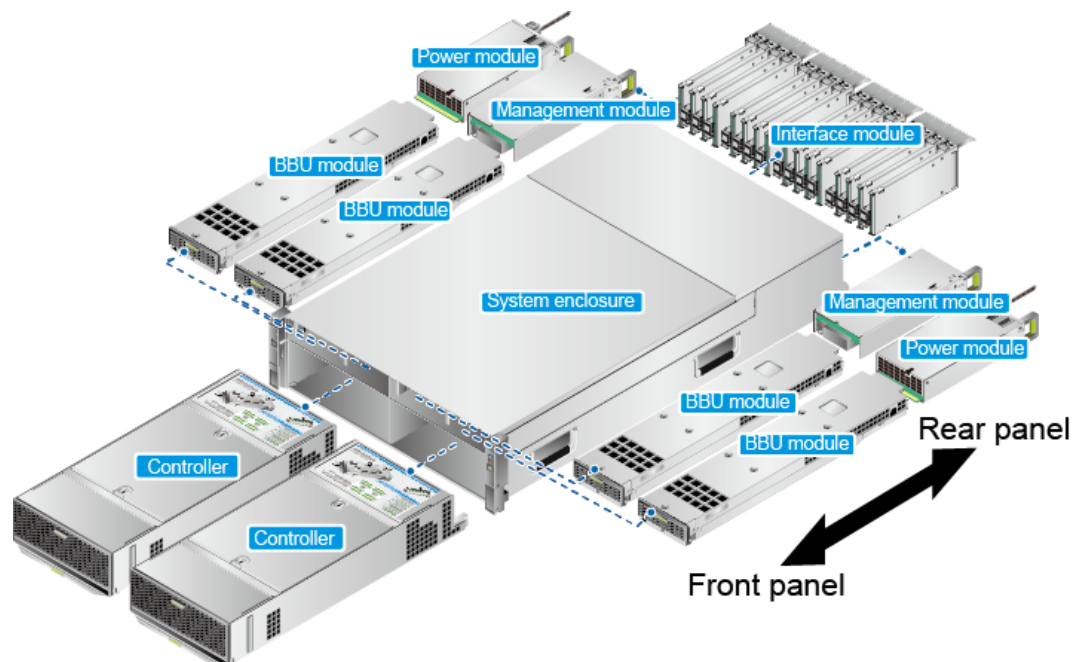
Figure 4-12 Overall structure of a controller enclosure
