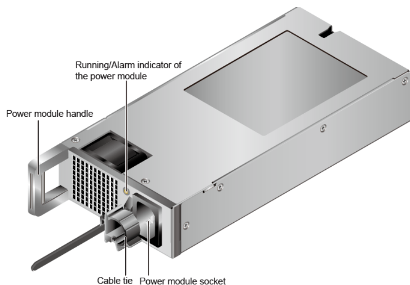
Figure 4-23 AC power module
