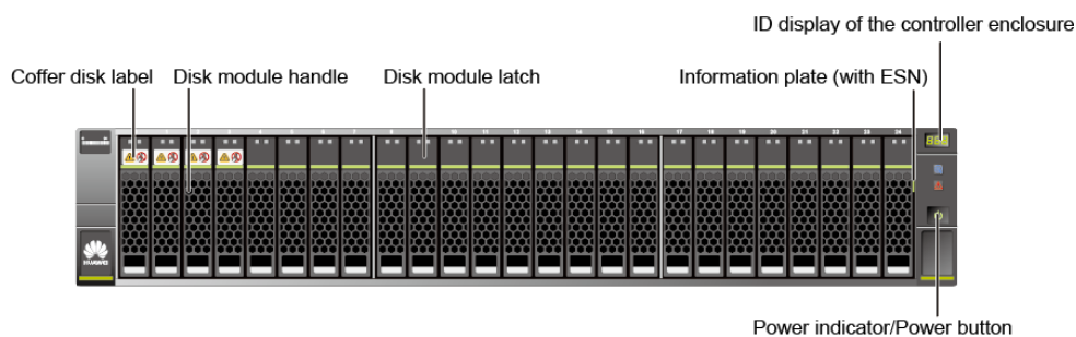
Figure 4-2 Front view of a 2 U 25-disk controller enclosure
