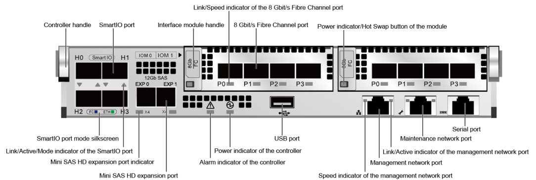
Figure 4-6 Ports of a controller
