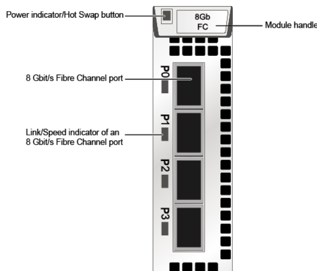
Figure 4-44 8 Gbit/s Fibre Channel interface module (four ports)
