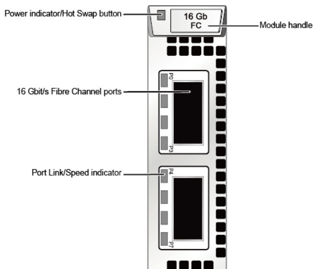
Figure 4-46 16 Gbit/s Fibre Channel interface module (eight ports)
