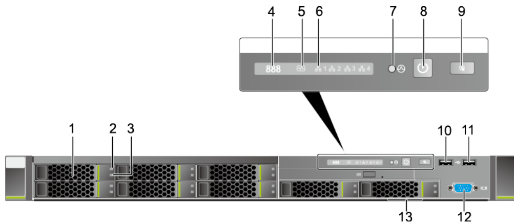
Figure 4-66 Front panel of the quorum server
