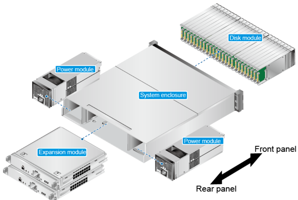
Figure 4-52 Overall structure of a disk enclosure
