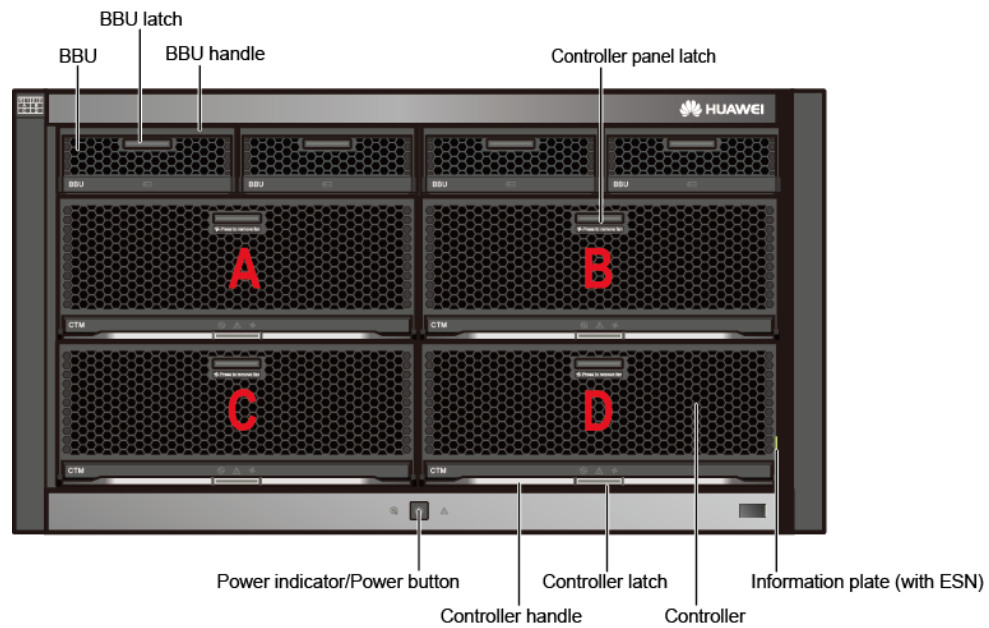
Figure 4-27 Front view of a controller enclosure
