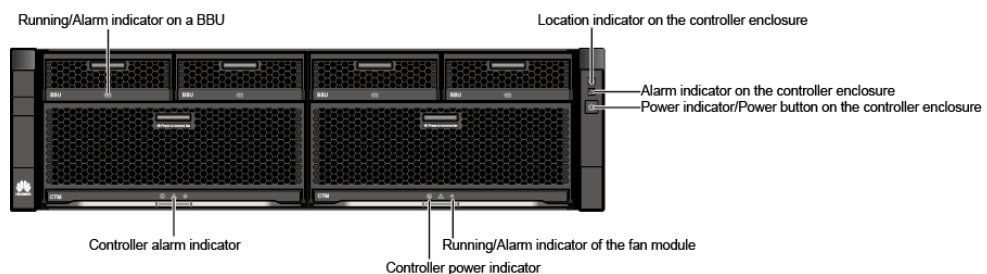
Figure 4-24 Indicators on the front panel of a controller enclosure
