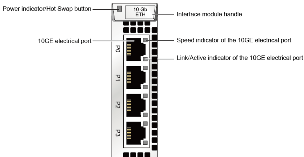
Figure 4-43 10GE electrical interface module
