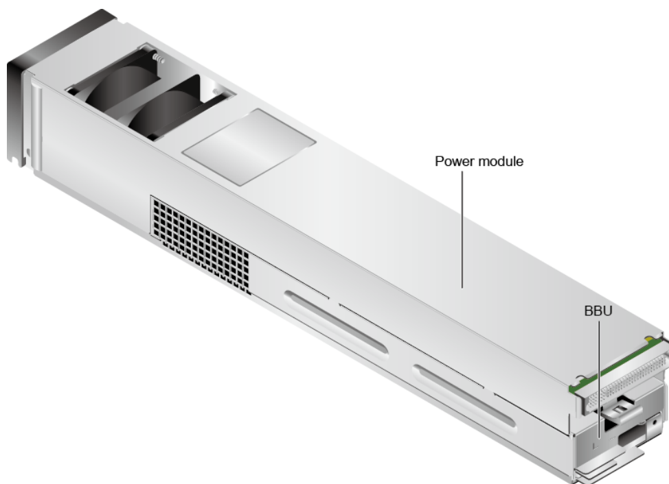
Figure 4-8 Rear view of a power-BBU module
