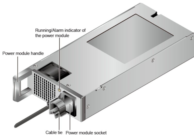
Figure 4-39 AC power module
