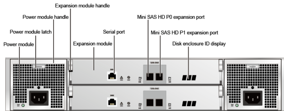
Figure 4-54 Rear view of a disk enclosure with the AC power module
