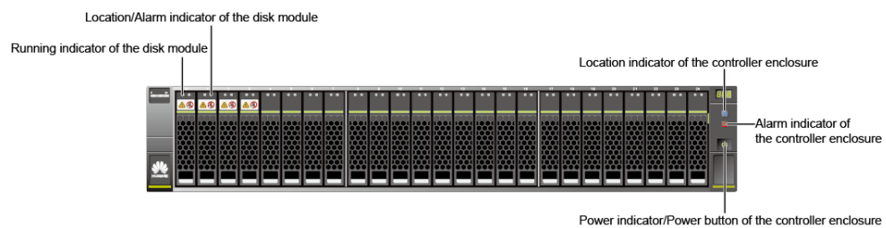
Figure 4-10 Indicators on the front panel of a 2 U 25-disk controller enclosure
