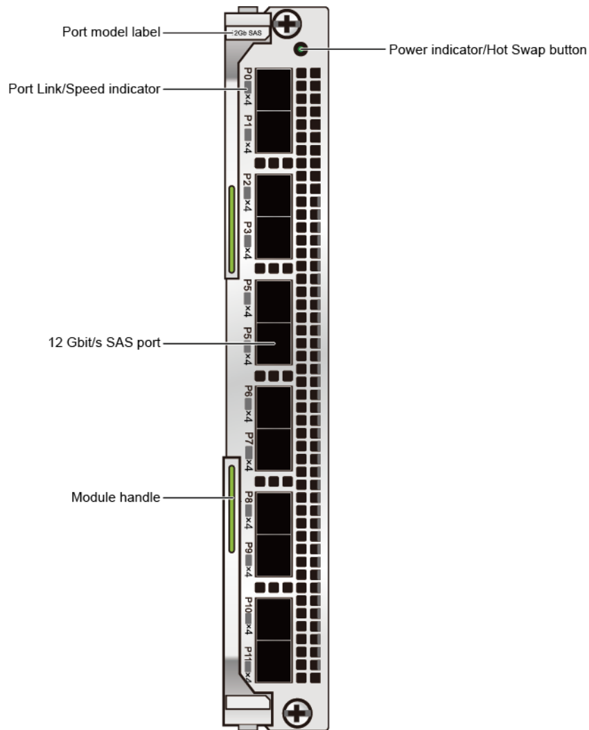
Figure 4-51 12 Gbit/s SAS shared expansion module
