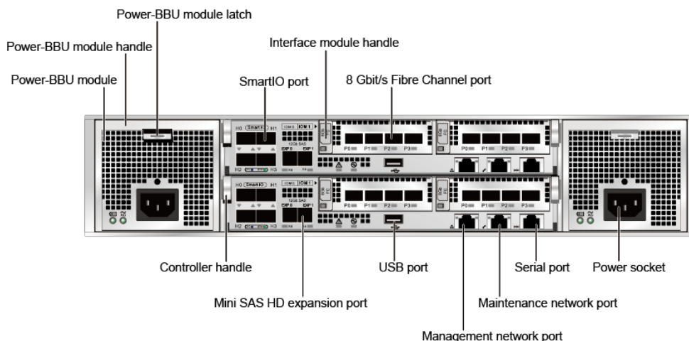
Figure 4-3 Rear view of a controller enclosure
