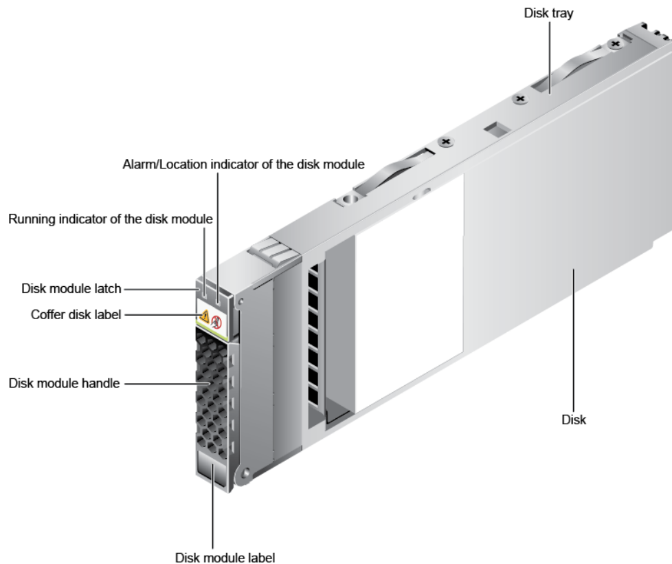
Figure 4-62 2.5-inch coffer disk
