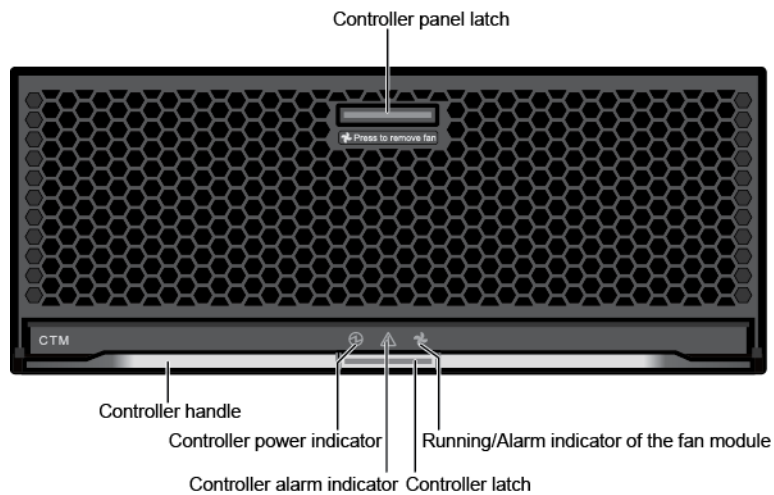
Figure 4-31 Front view of a controller
