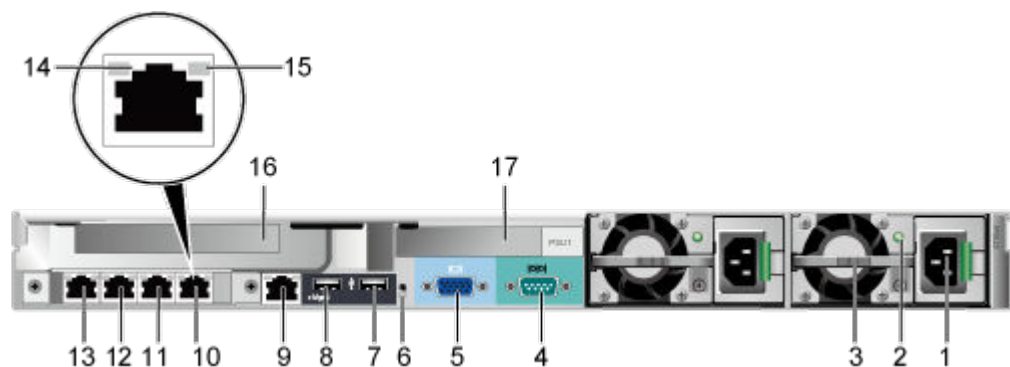
Figure 4-67 Rear view of the quorum server
