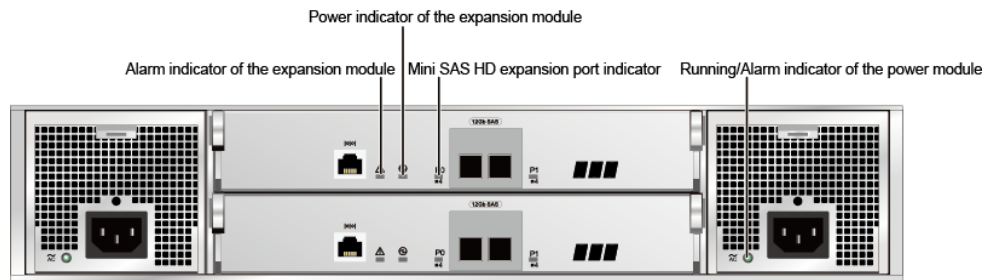
Figure 4-61 Indicators on the rear panel of a disk enclosure
