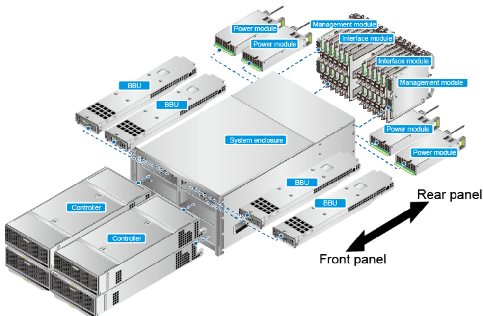
Figure 4-26 Overall structure of a controller enclosure
