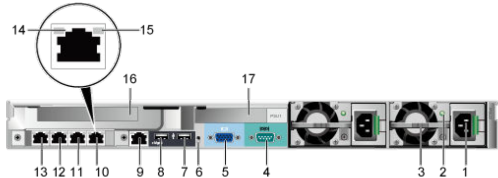
Figure 4-44 Rear view of the quorum server
