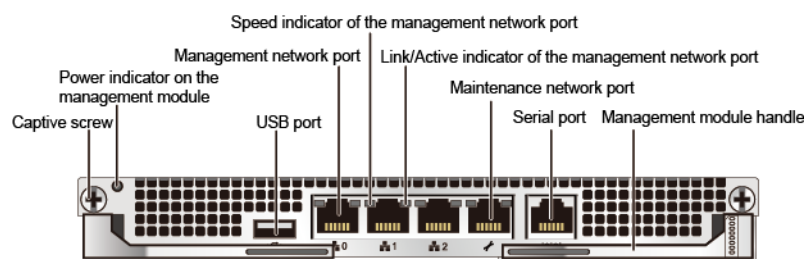
Figure 4-14 Management module
