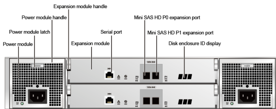
Figure 4-29 Rear view of a disk enclosure with the AC power module
