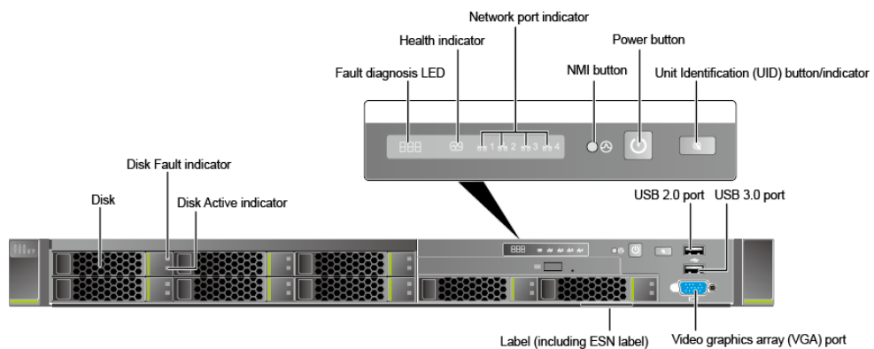
Figure 4-41 Front Panel of the SVP
