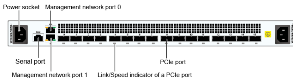
Figure 4-40 Rear view of a data switch
