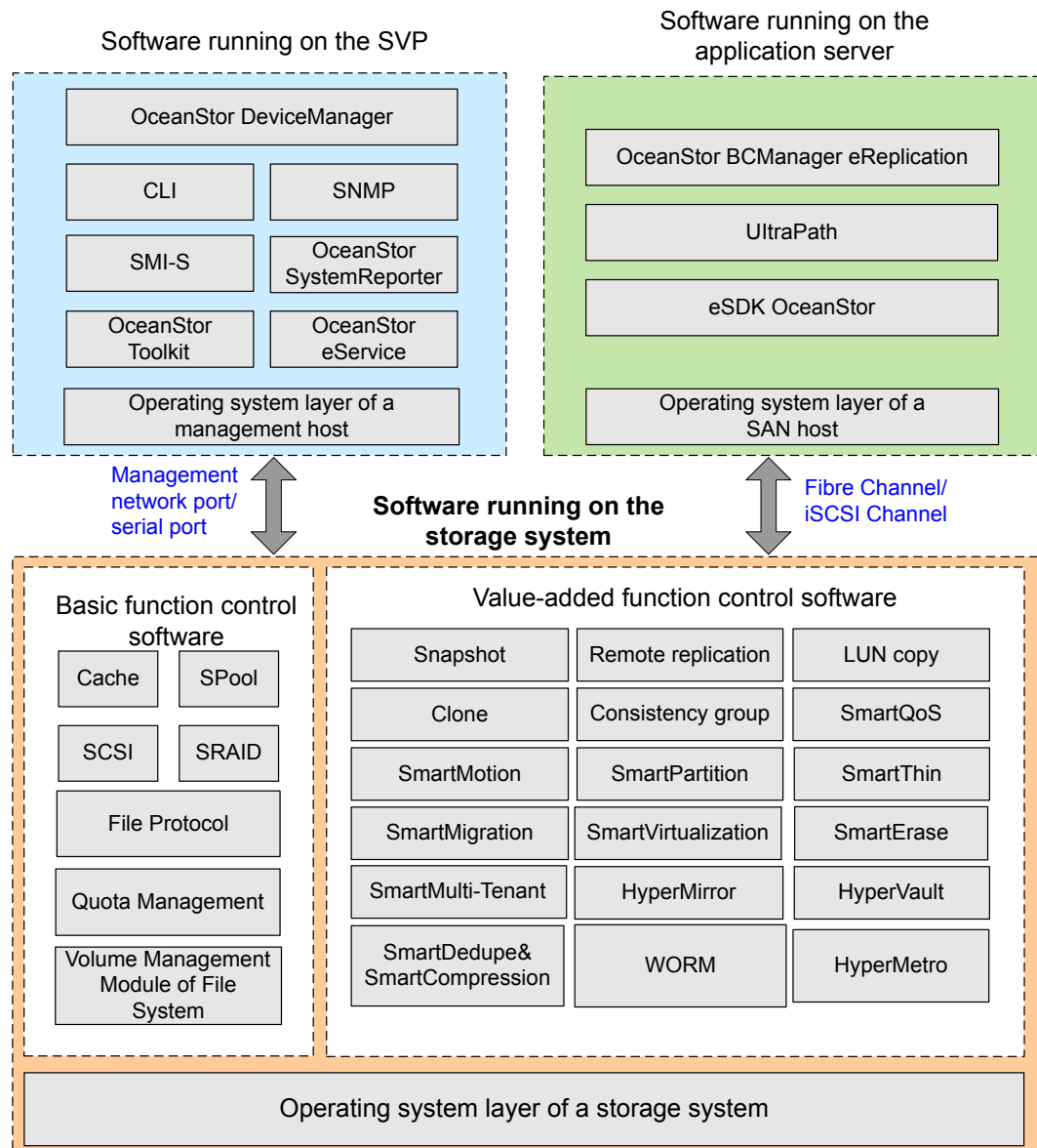
Figure 5-1 Software architecture of the OceanStor 18500F V5 and 18800F V5 mission critical storage system
