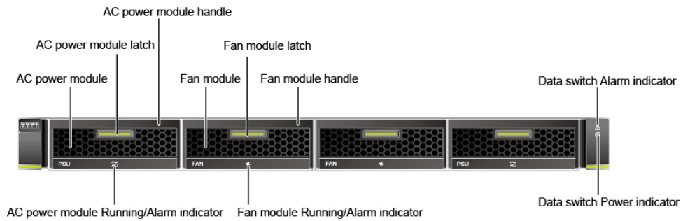
Figure 4-39 Front view of data switch
