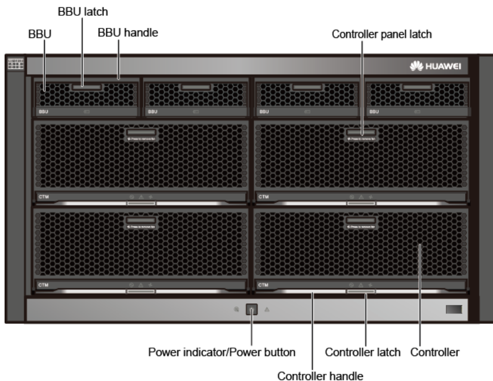
Figure 4-3 Front view of an engine
