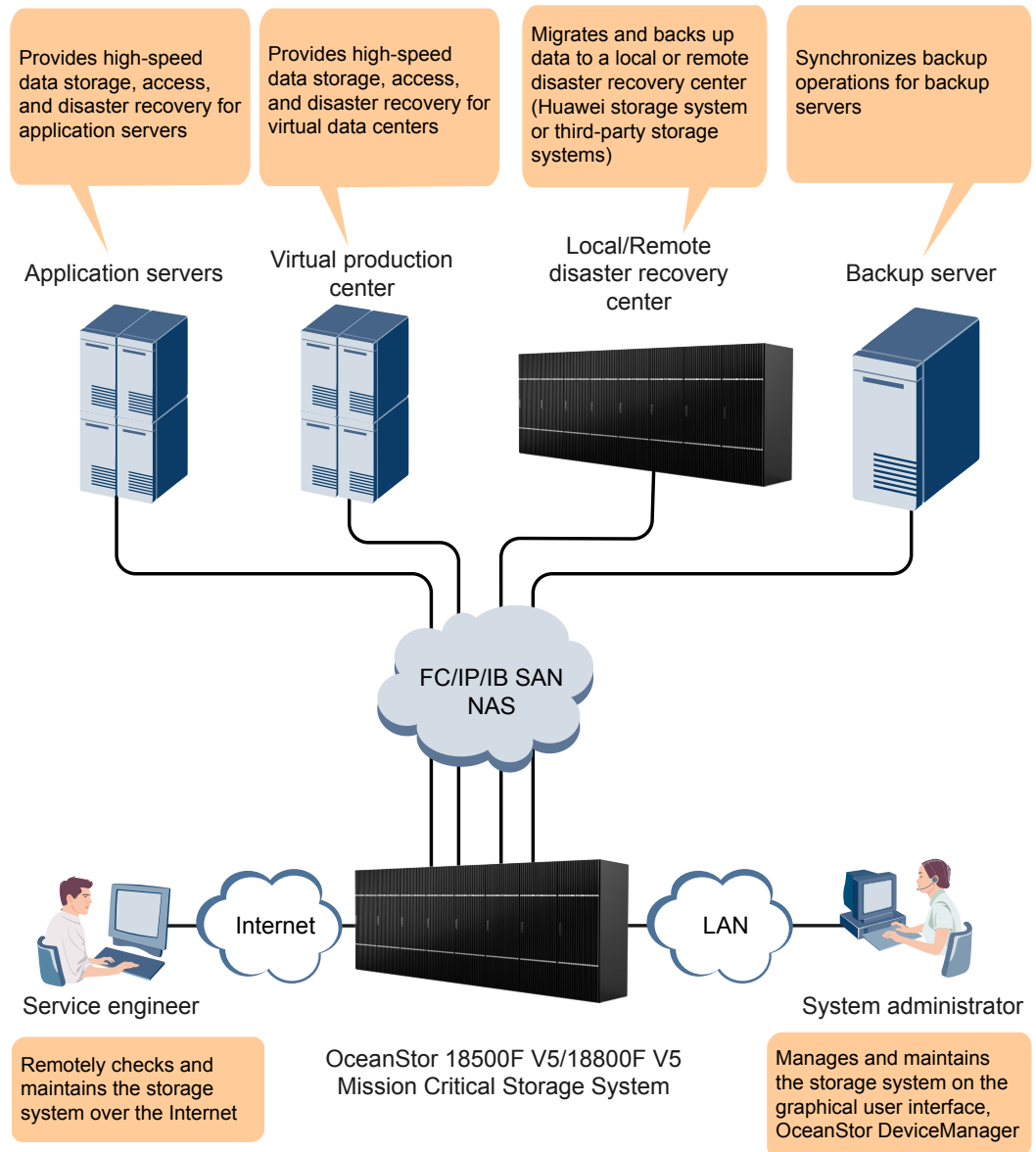
Figure 1-2 Role and applications of OceanStor 18500F V5 and 18800F V5 mission critical storage system in the network
