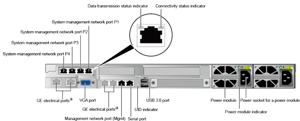
Figure 4-42 Rear view of the SVP
