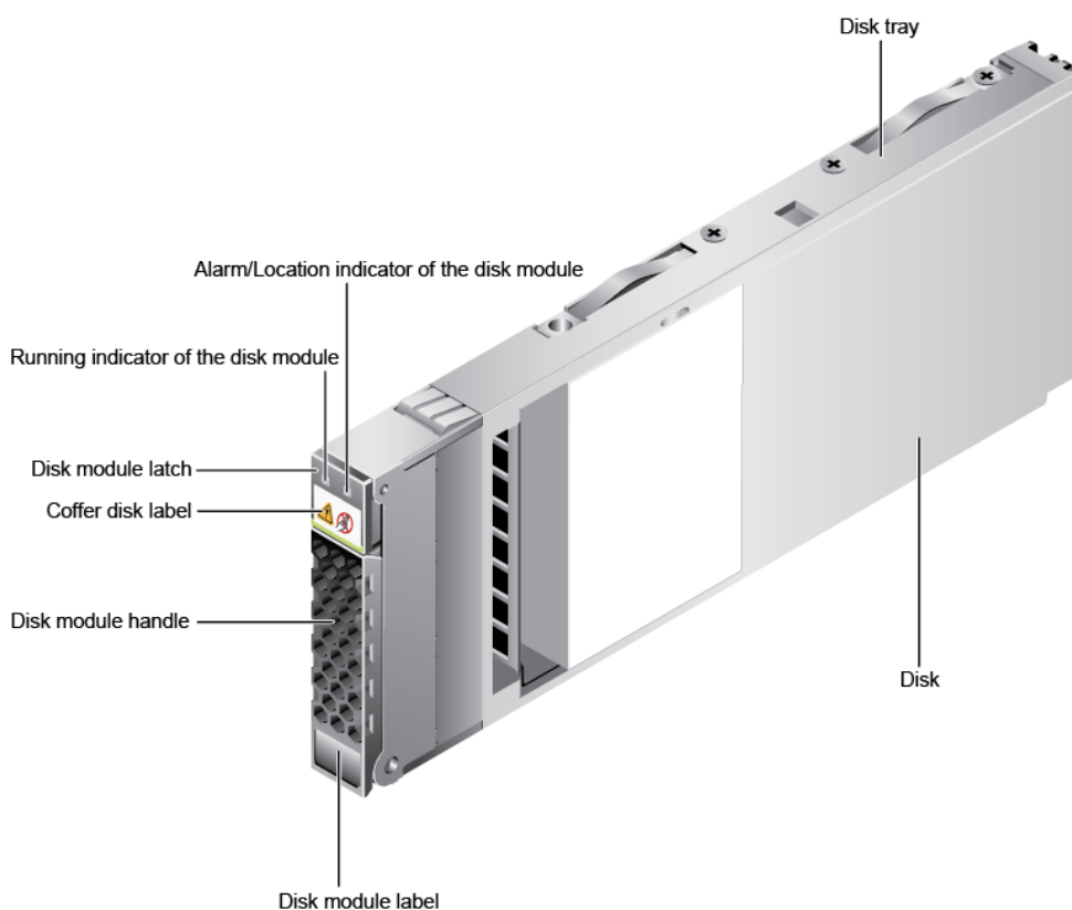
Figure 4-37 2.5-inch coffer disk
