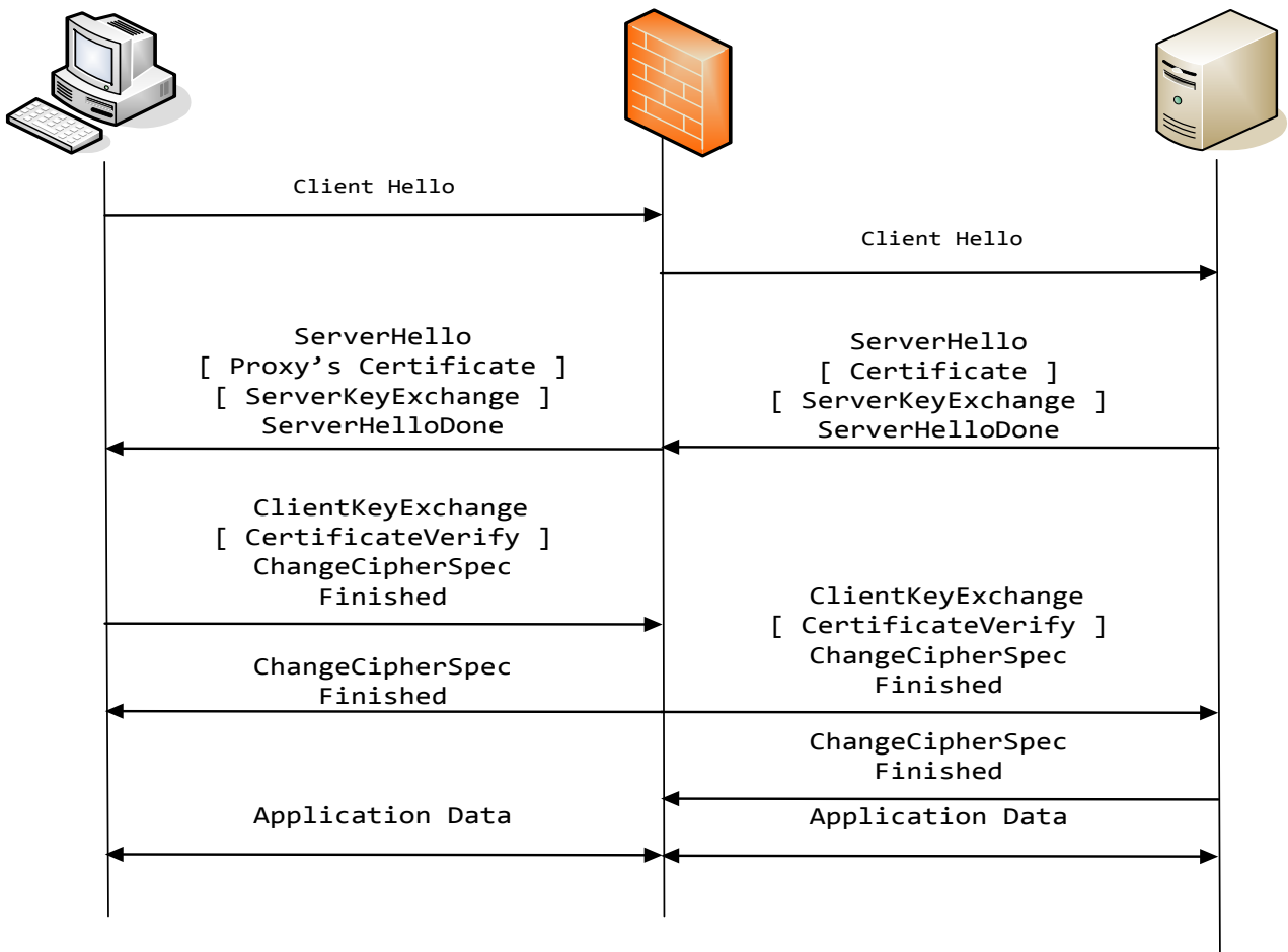
Figure 2-2 SSL proxy process
