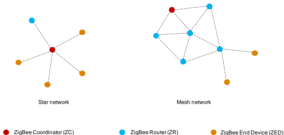
Figure 2-6 ZigBee network topologies
