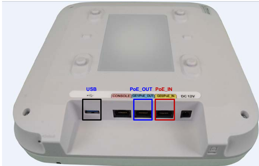
Figure 2-2 Physical interface 1 of an IoT AP
