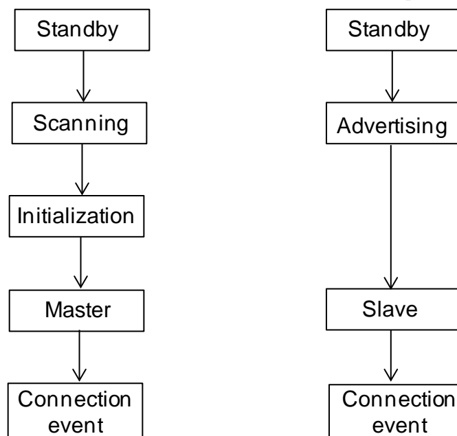
Figure 2-5 BLE master-slave communication connection process
