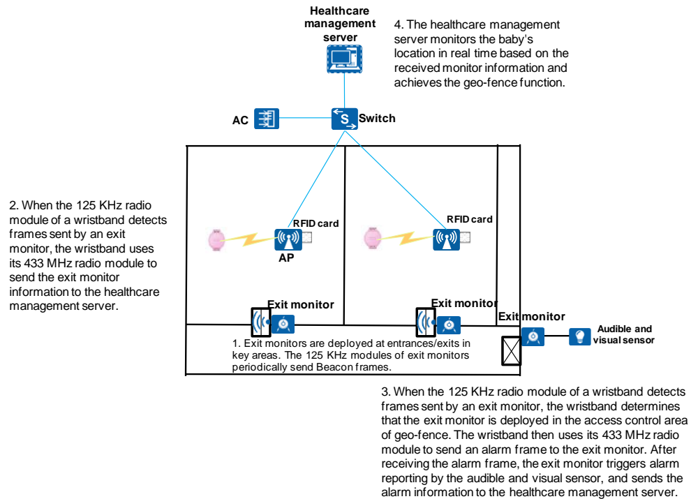
Figure 3-5 Baby theft prevention process
