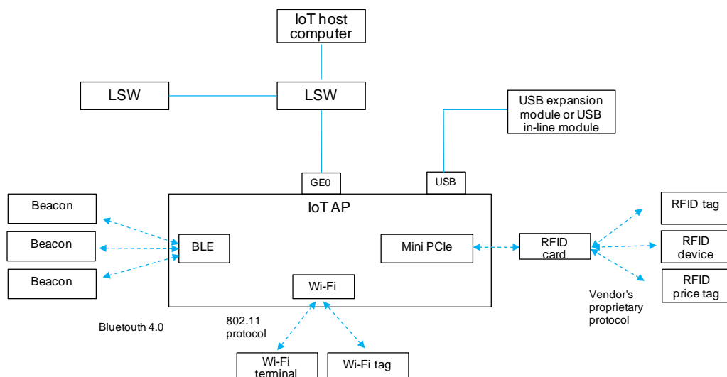
Figure 2-1 Technical architecture of an IoT AP
