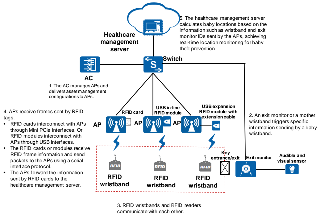
Figure 3-3 Networking diagram for baby theft prevention
