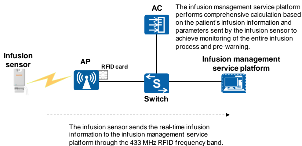
Figure 3-6 Infusion management diagram
