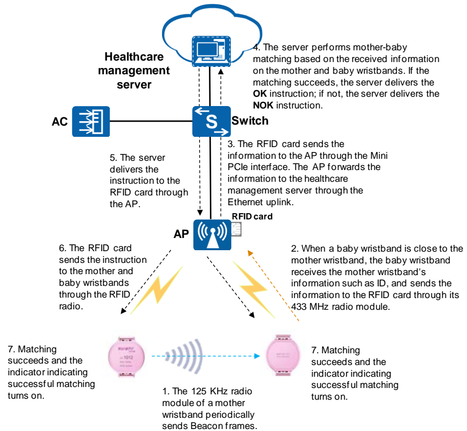
Figure 3-4 Mother-baby matching process
