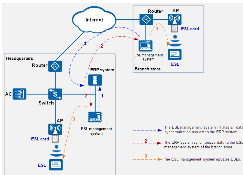
Figure 3-7 ESL working process
