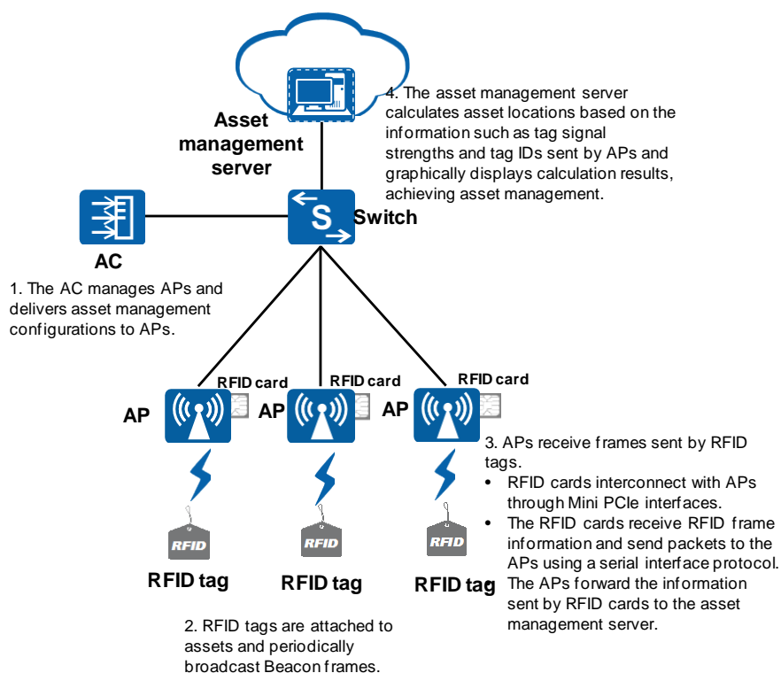
Figure 3-2 Networking diagram for RFID-based asset management
