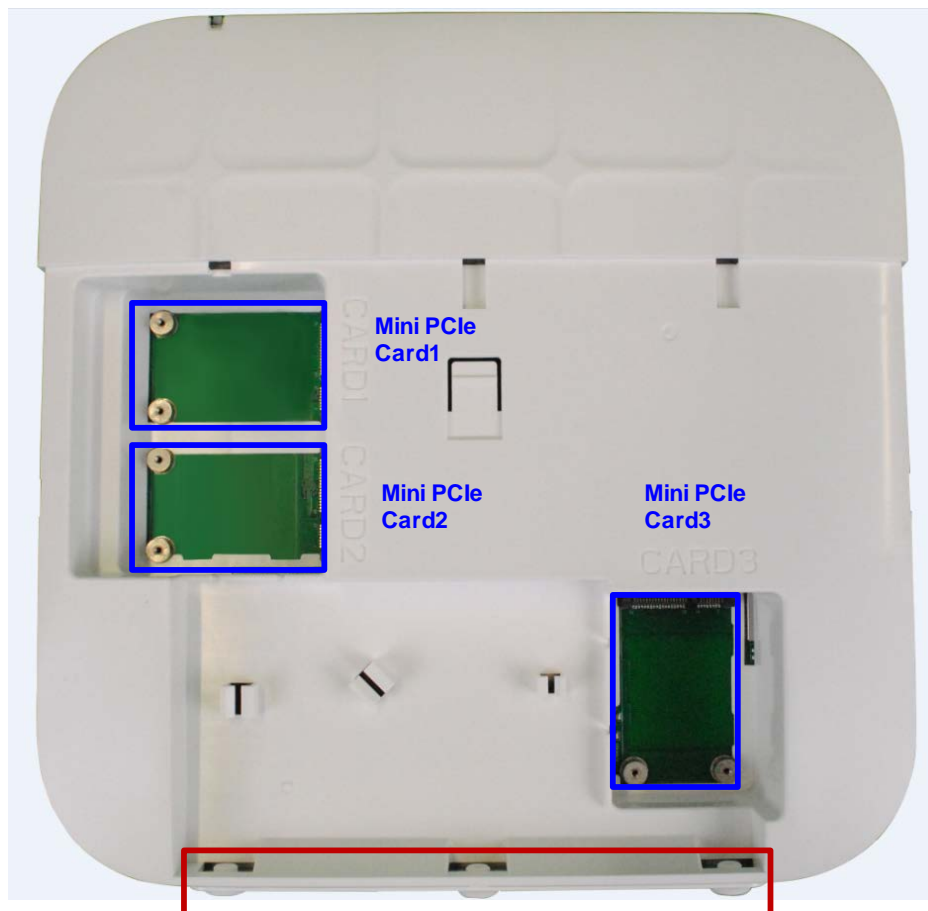
Figure 2-3 Physical interface 2 of an IoT AP
