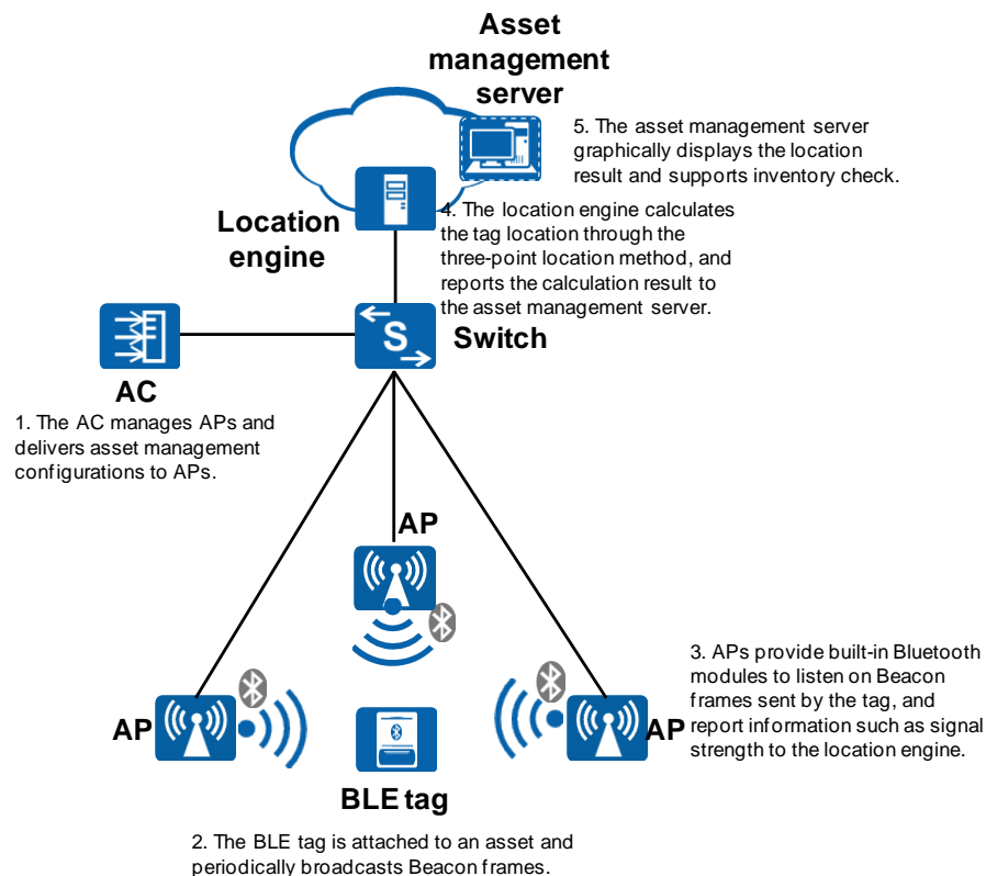
Figure 3-1 Networking diagram for BLE-based asset management
