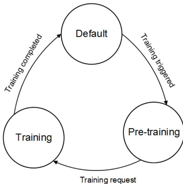
Figure 2-4 Working state switching of antennas
