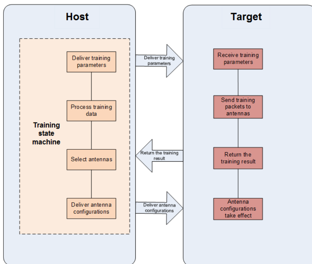
Figure 2-5 Antenna training and selection
