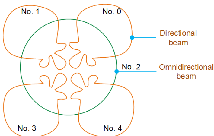
Figure 2-3 Five beams of a small antenna
