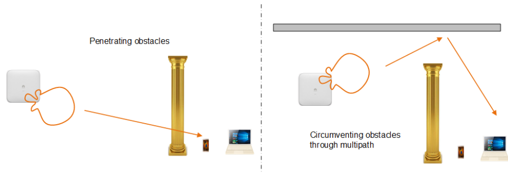
Figure 4-2 Smart antenna beam selection when obstacles exist
