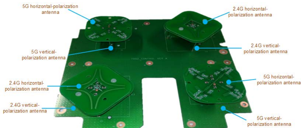
Figure 2-2 Smart antenna array arrangement
