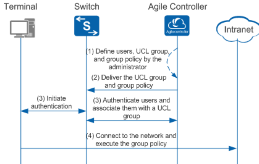
Figure 2-2 Implementation of free mobility
