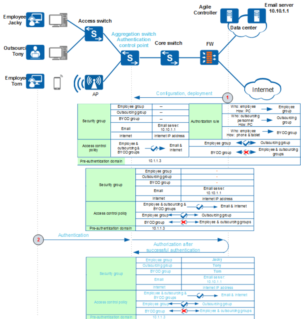
Figure 3-1 Free mobility deployment in campus access scenarios
